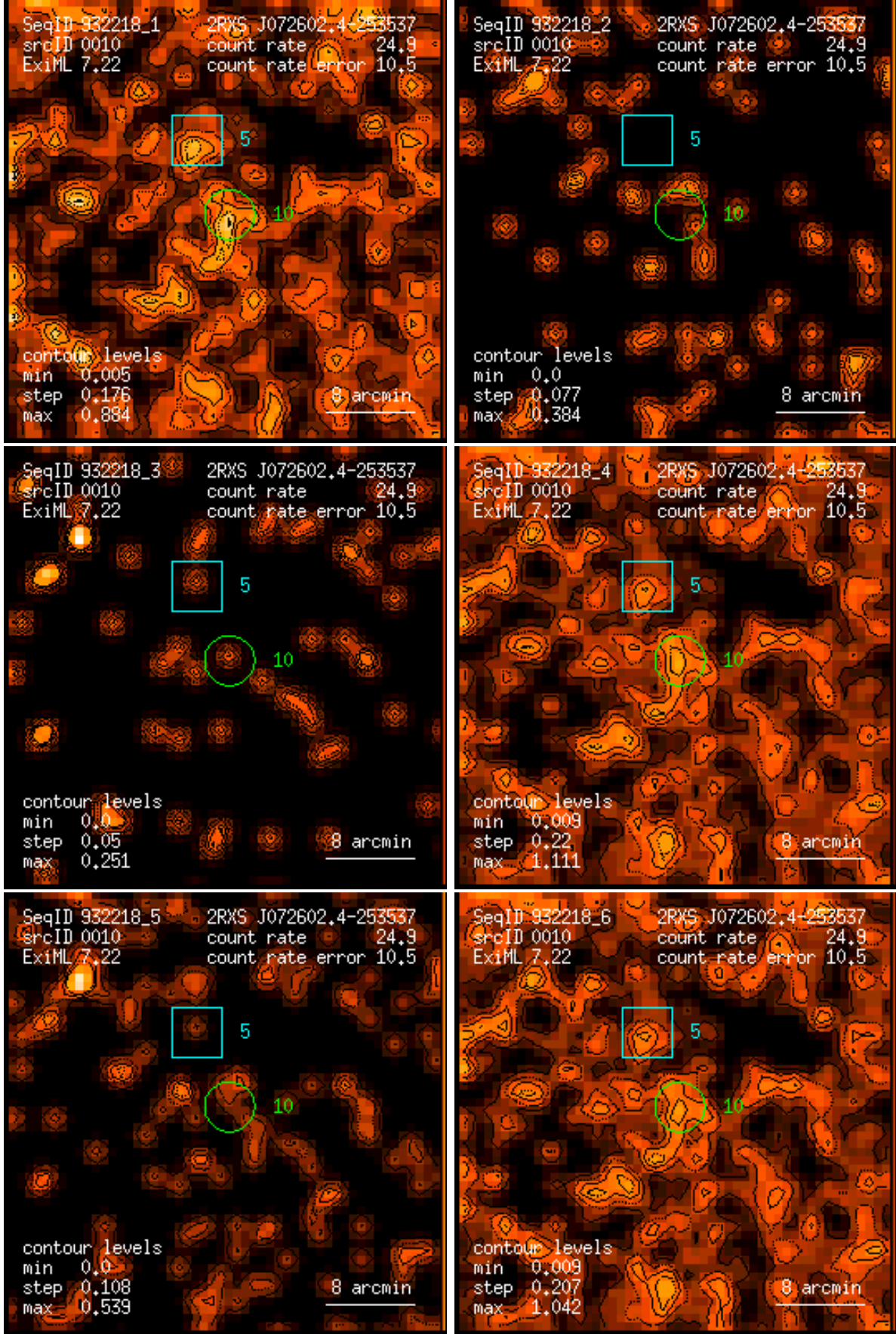
Figure 10: RASS 932218: detection 0010: band rate images, Gaussian filter: (1) PSPC channels 11 – 41, (2) 52 – 90, (3) 91 – 201, (4) 11 – 235, (5) 52 – 201, (6) 11 – 201. Broad band rates in counts/ks. Band rate contour levels in counts/ks/arcmin 2 .
