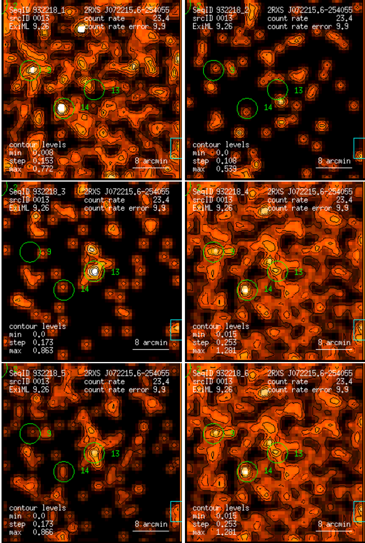
Figure 13: RASS 932218: detection 0013: band rate images, Gaussian filter: (1) PSPC channels 11 – 41, (2) 52 – 90, (3) 91 – 201, (4) 11 – 235, (5) 52 – 201, (6) 11 – 201. Broad band rates in counts/ks. Band rate contour levels in counts/ks/arcmin 2 .
