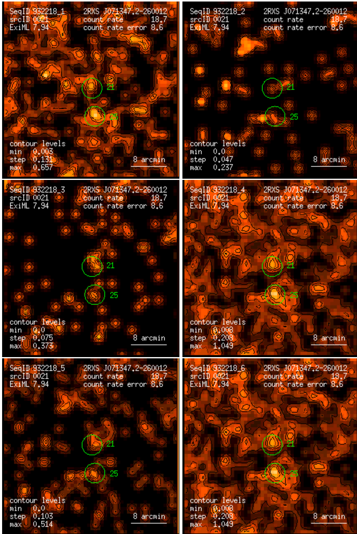
Figure 21: RASS 932218: detection 0021: band rate images, Gaussian filter: (1) PSPC channels 11 – 41, (2) 52 – 90, (3) 91 – 201, (4) 11 – 235, (5) 52 – 201, (6) 11 – 201. Broad band rates in counts/ks. Band rate contour levels in counts/ks/arcmin 2 .
