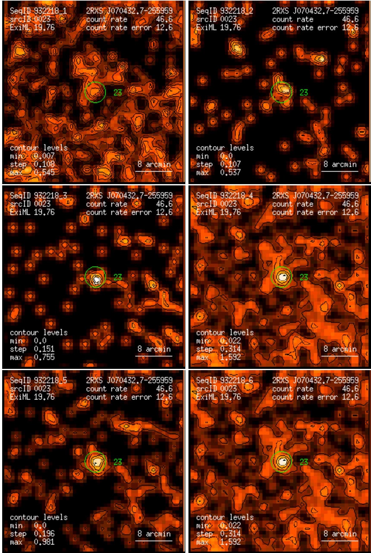
Figure 23: RASS 932218: detection 0023: band rate images, Gaussian filter: (1) PSPC channels 11 – 41, (2) 52 – 90, (3) 91 – 201, (4) 11 – 235, (5) 52 – 201, (6) 11 – 201. Broad band rates in counts/ks. Band rate contour levels in counts/ks/arcmin 2 .
