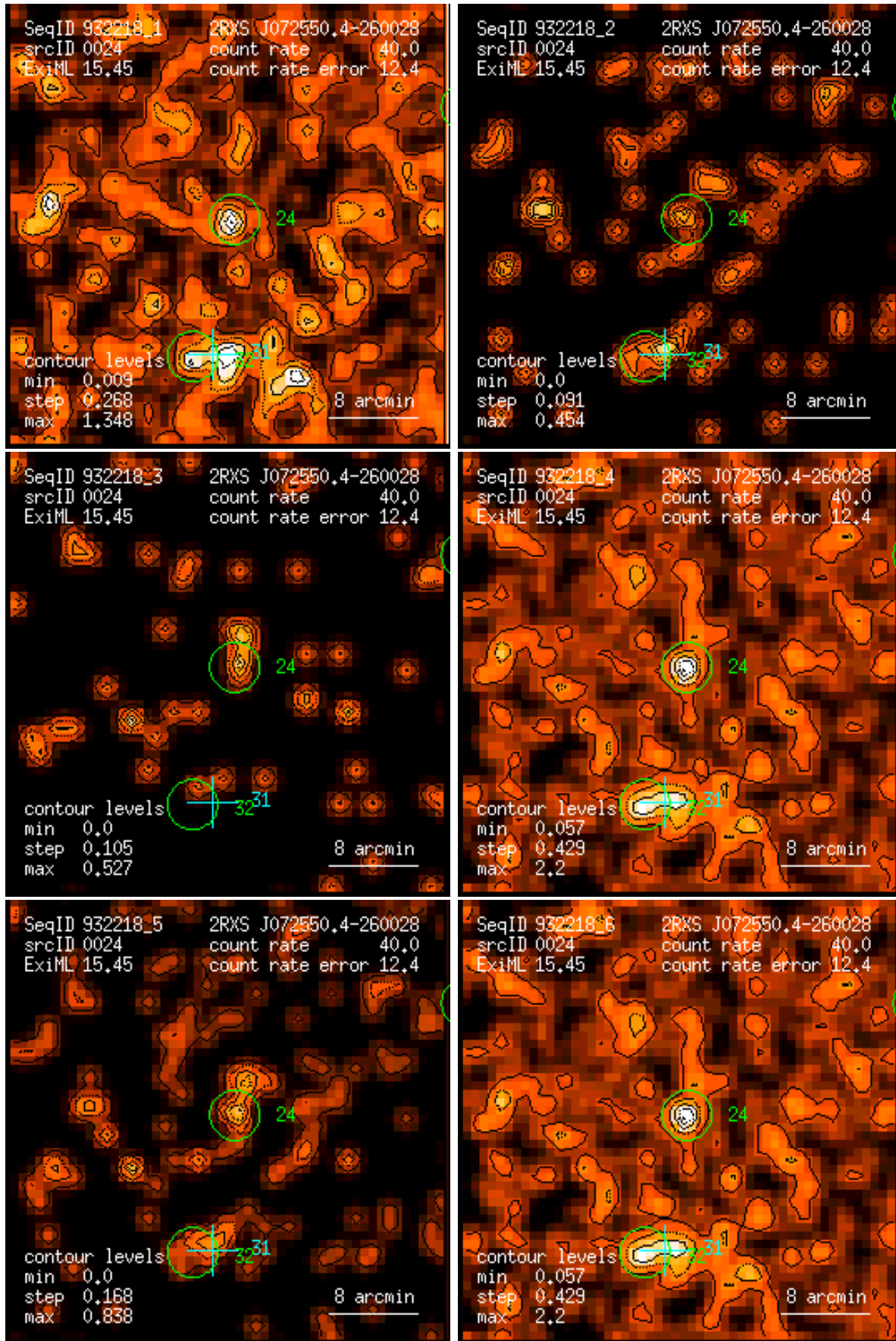
Figure 24: RASS 932218: detection 0024: band rate images, Gaussian filter: (1) PSPC channels 11 – 41, (2) 52 – 90, (3) 91 – 201, (4) 11 – 235, (5) 52 – 201, (6) 11 – 201. Broad band rates in counts/ks. Band rate contour levels in counts/ks/arcmin 2 .
