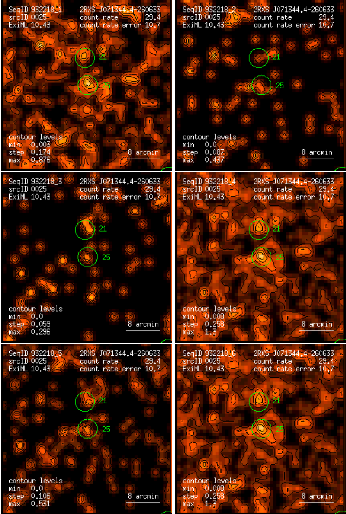
Figure 25: RASS 932218: detection 0025: band rate images, Gaussian filter: (1) PSPC channels 11 – 41, (2) 52 – 90, (3) 91 – 201, (4) 11 – 235, (5) 52 – 201, (6) 11 – 201. Broad band rates in counts/ks. Band rate contour levels in counts/ks/arcmin 2 .
