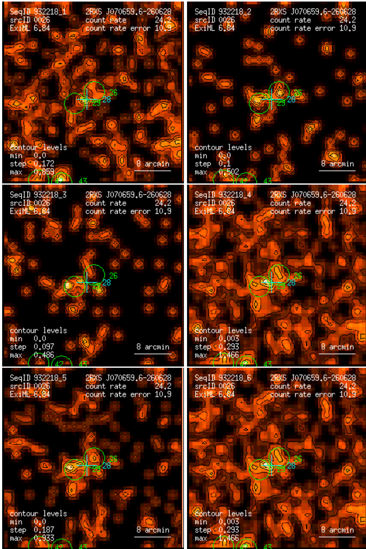
Figure 26: RASS 932218: detection 0026: band rate images, Gaussian filter: (1) PSPC channels 11 – 41, (2) 52 – 90, (3) 91 – 201, (4) 11 – 235, (5) 52 – 201, (6) 11 – 201. Broad band rates in counts/ks. Band rate contour levels in counts/ks/arcmin 2 .
