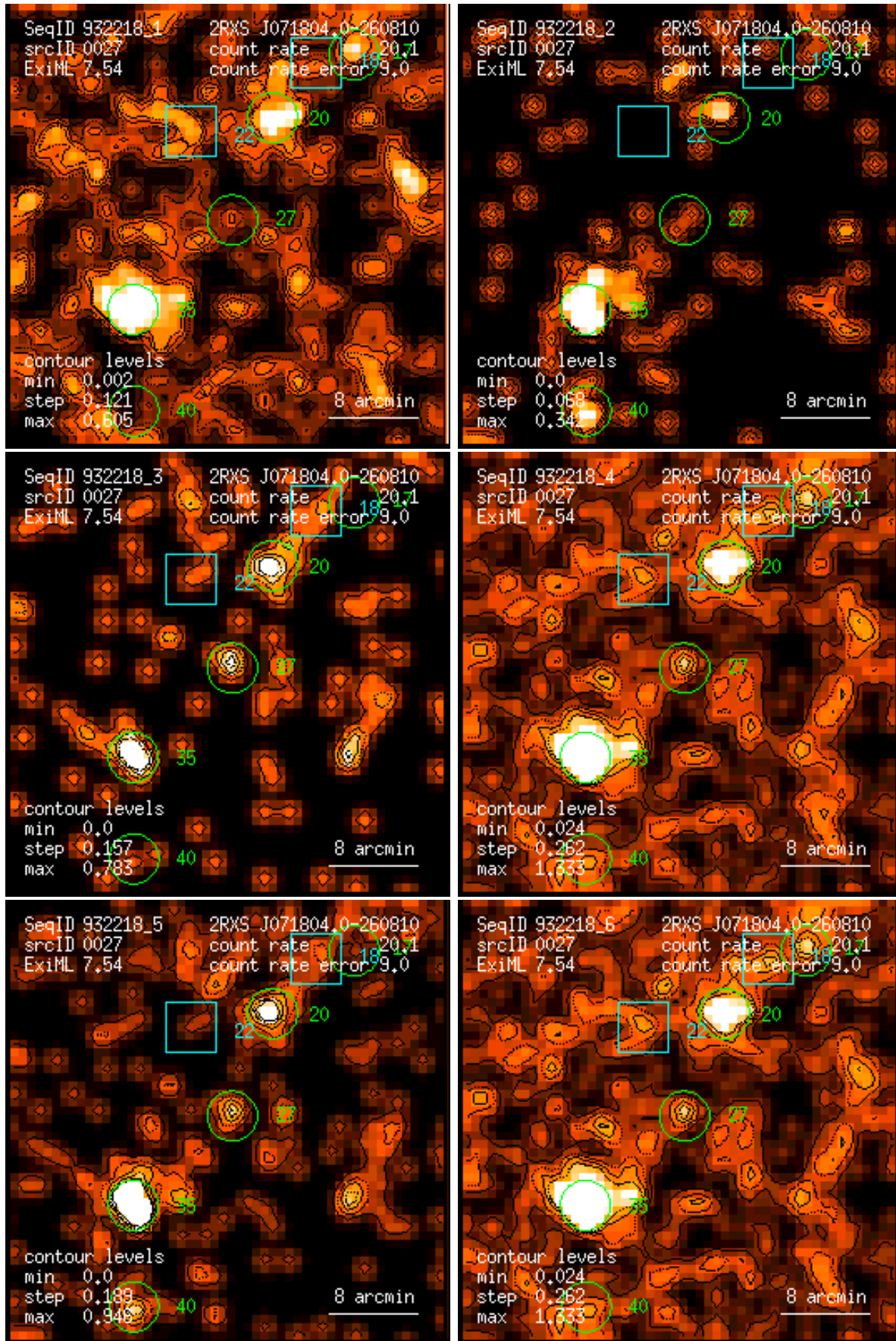
Figure 27: RASS 932218: detection 0027: band rate images, Gaussian filter: (1) PSPC channels 11 – 41, (2) 52 – 90, (3) 91 – 201, (4) 11 – 235, (5) 52 – 201, (6) 11 – 201. Broad band rates in counts/ks. Band rate contour levels in counts/ks/arcmin 2 .
