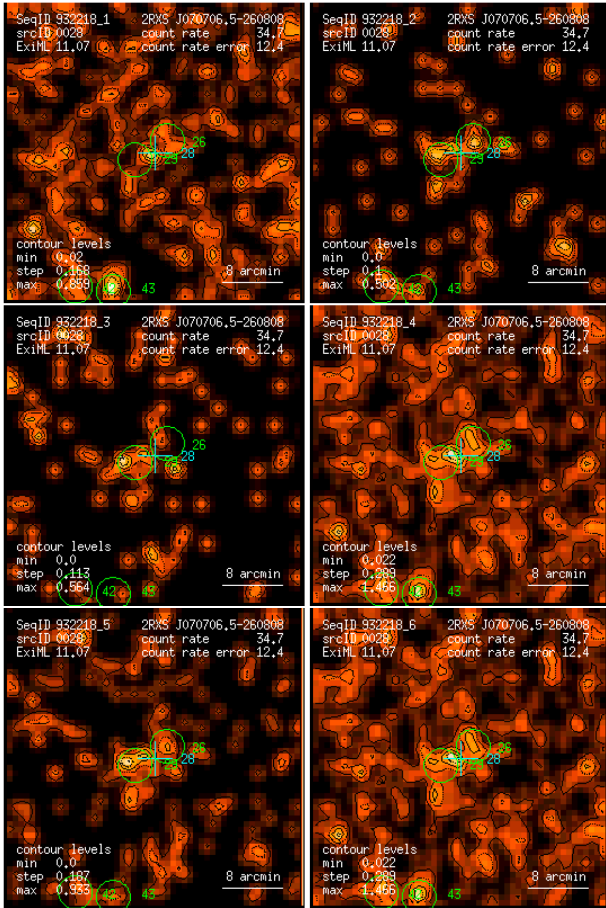
Figure 28: RASS 932218: detection 0028: band rate images, Gaussian filter: (1) PSPC channels 11 – 41, (2) 52 – 90, (3) 91 – 201, (4) 11 – 235, (5) 52 – 201, (6) 11 – 201. Broad band rates in counts/ks. Band rate contour levels in counts/ks/arcmin 2 .
