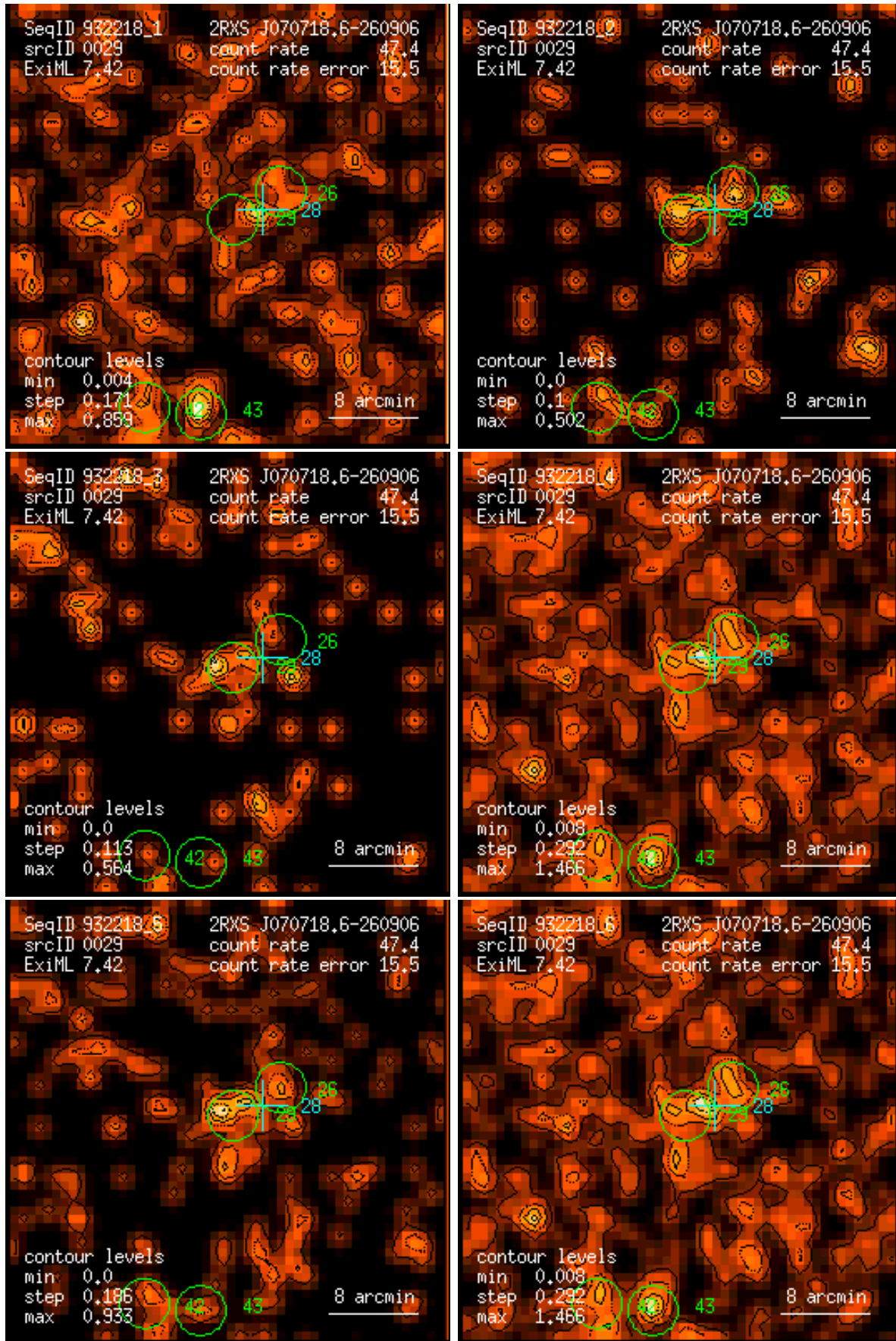
Figure 29: RASS 932218: detection 0029: band rate images, Gaussian filter: (1) PSPC channels 11 – 41, (2) 52 – 90, (3) 91 – 201, (4) 11 – 235, (5) 52 – 201, (6) 11 – 201. Broad band rates in counts/ks. Band rate contour levels in counts/ks/arcmin 2 .
