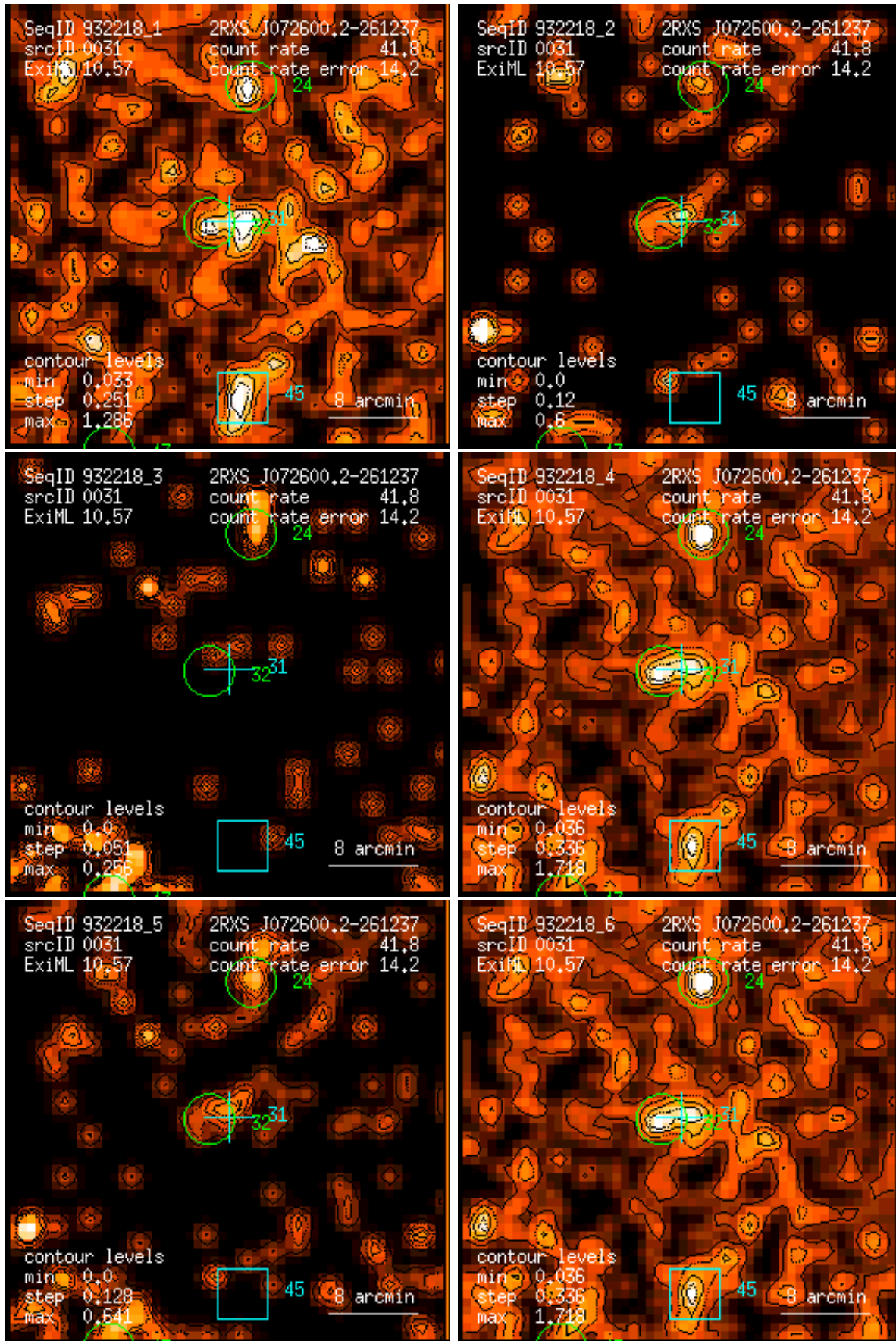
Figure 31: RASS 932218: detection 0031: band rate images, Gaussian filter: (1) PSPC channels 11 – 41, (2) 52 – 90, (3) 91 – 201, (4) 11 – 235, (5) 52 – 201, (6) 11 – 201. Broad band rates in counts/ks. Band rate contour levels in counts/ks/arcmin 2 .
