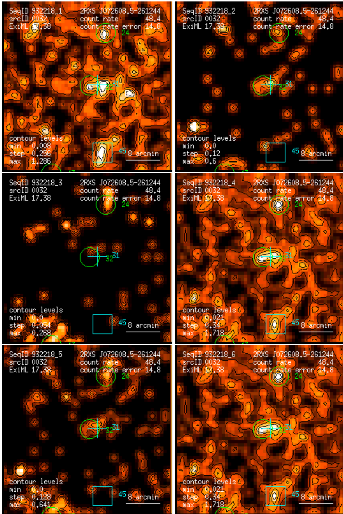
Figure 32: RASS 932218: detection 0032: band rate images, Gaussian filter: (1) PSPC channels 11 – 41, (2) 52 – 90, (3) 91 – 201, (4) 11 – 235, (5) 52 – 201, (6) 11 – 201. Broad band rates in counts/ks. Band rate contour levels in counts/ks/arcmin 2 .
