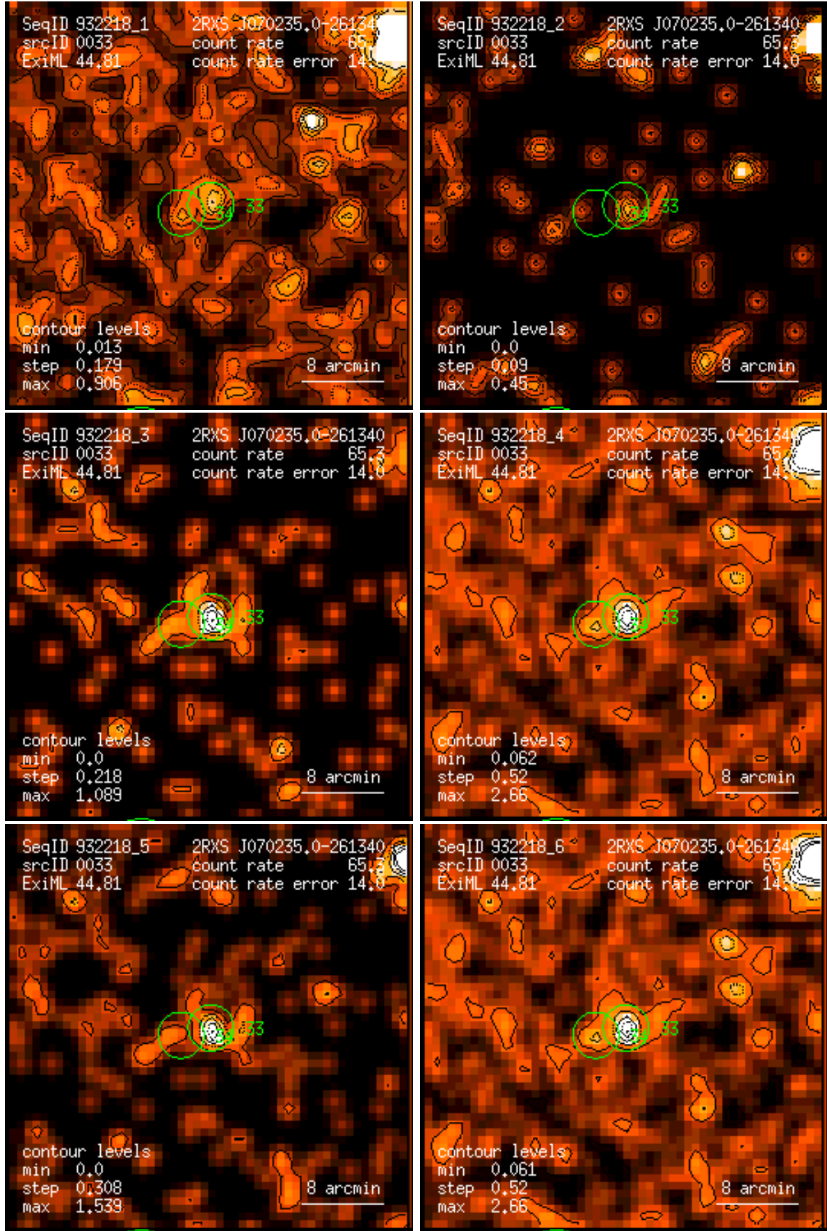
Figure 33: RASS 932218: detection 0033: band rate images, Gaussian filter: (1) PSPC channels 11 – 41, (2) 52 – 90, (3) 91 – 201, (4) 11 – 235, (5) 52 – 201, (6) 11 – 201. Broad band rates in counts/ks. Band rate contour levels in counts/ks/arcmin 2 .
