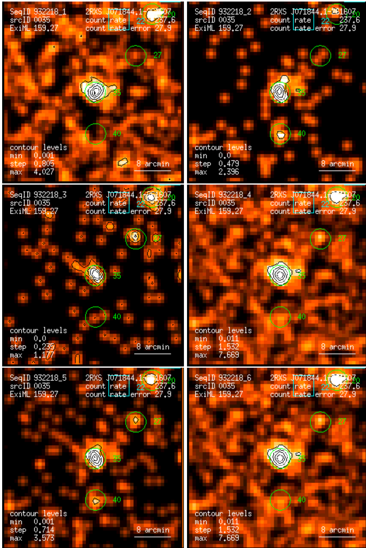
Figure 35: RASS 932218: detection 0035: band rate images, Gaussian filter: (1) PSPC channels 11 – 41, (2) 52 – 90, (3) 91 – 201, (4) 11 – 235, (5) 52 – 201, (6) 11 – 201. Broad band rates in counts/ks. Band rate contour levels in counts/ks/arcmin 2 .
