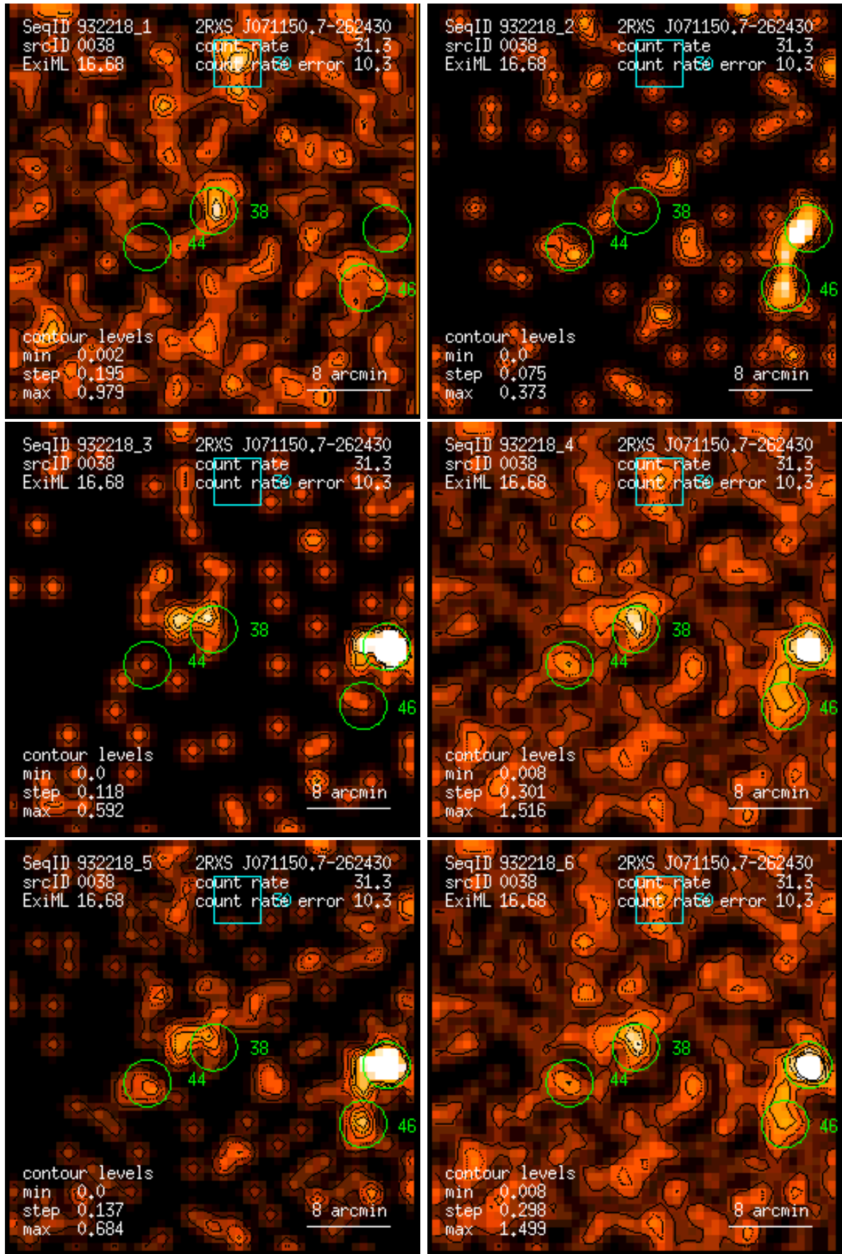
Figure 38: RASS 932218: detection 0038: band rate images, Gaussian filter: (1) PSPC channels 11 – 41, (2) 52 – 90, (3) 91 – 201, (4) 11 – 235, (5) 52 – 201, (6) 11 – 201. Broad band rates in counts/ks. Band rate contour levels in counts/ks/arcmin 2 .
