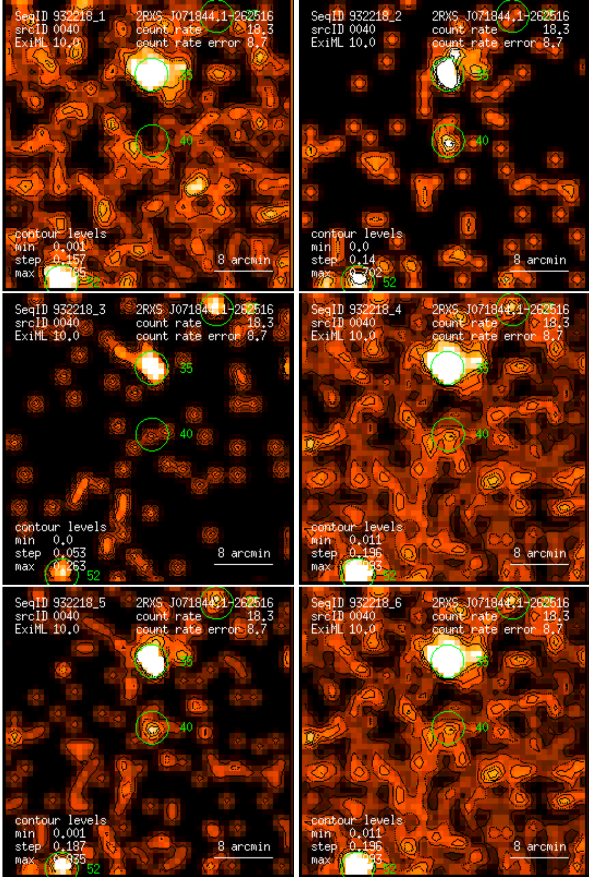
Figure 40: RASS 932218: detection 0040: band rate images, Gaussian filter: (1) PSPC channels 11 – 41, (2) 52 – 90, (3) 91 – 201, (4) 11 – 235, (5) 52 – 201, (6) 11 – 201. Broad band rates in counts/ks. Band rate contour levels in counts/ks/arcmin 2 .
