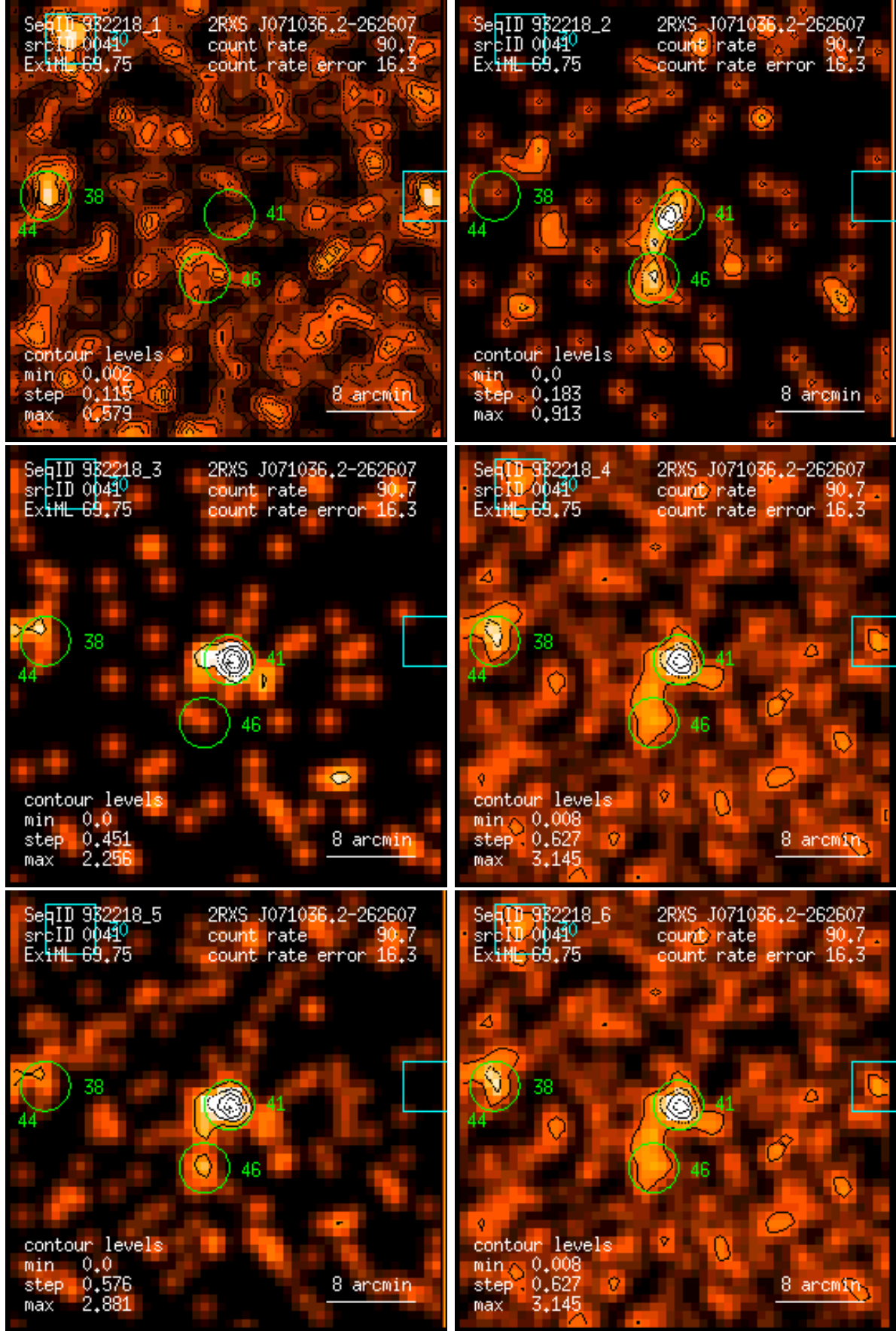
Figure 41: RASS 932218: detection 0041: band rate images, Gaussian filter: (1) PSPC channels 11 – 41, (2) 52 – 90, (3) 91 – 201, (4) 11 – 235, (5) 52 – 201, (6) 11 – 201. Broad band rates in counts/ks. Band rate contour levels in counts/ks/arcmin 2 .
