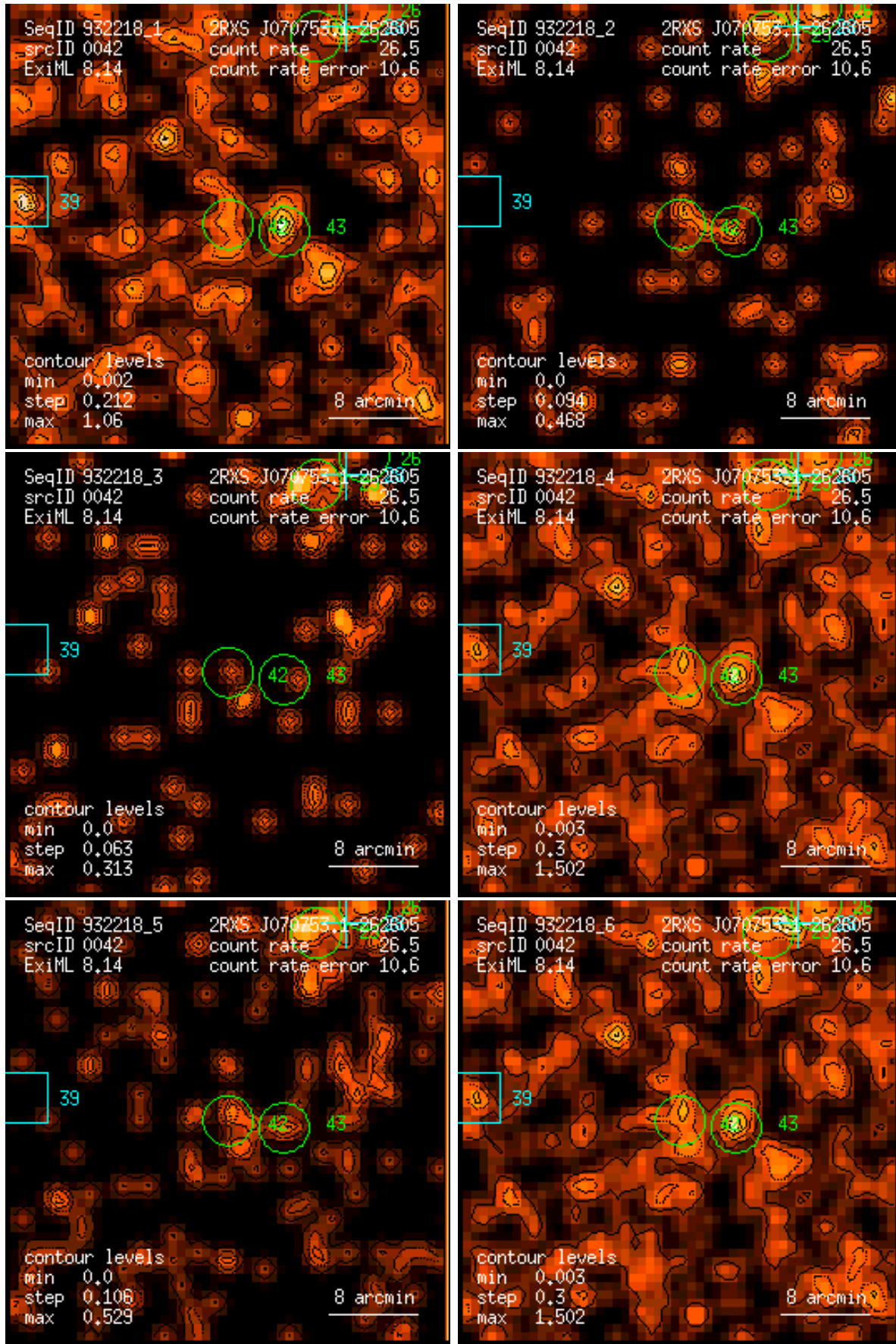
Figure 42: RASS 932218: detection 0042: band rate images, Gaussian filter: (1) PSPC channels 11 – 41, (2) 52 – 90, (3) 91 – 201, (4) 11 – 235, (5) 52 – 201, (6) 11 – 201. Broad band rates in counts/ks. Band rate contour levels in counts/ks/arcmin 2 .
