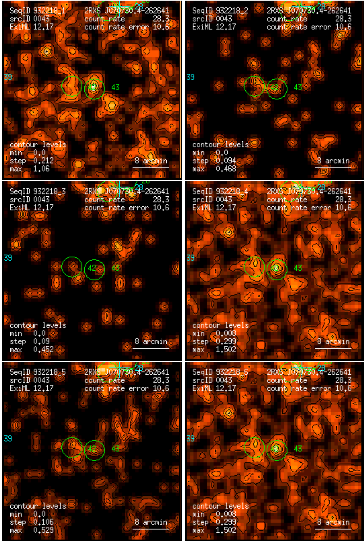
Figure 43: RASS 932218: detection 0043: band rate images, Gaussian filter: (1) PSPC channels 11 – 41, (2) 52 – 90, (3) 91 – 201, (4) 11 – 235, (5) 52 – 201, (6) 11 – 201. Broad band rates in counts/ks. Band rate contour levels in counts/ks/arcmin 2 .
