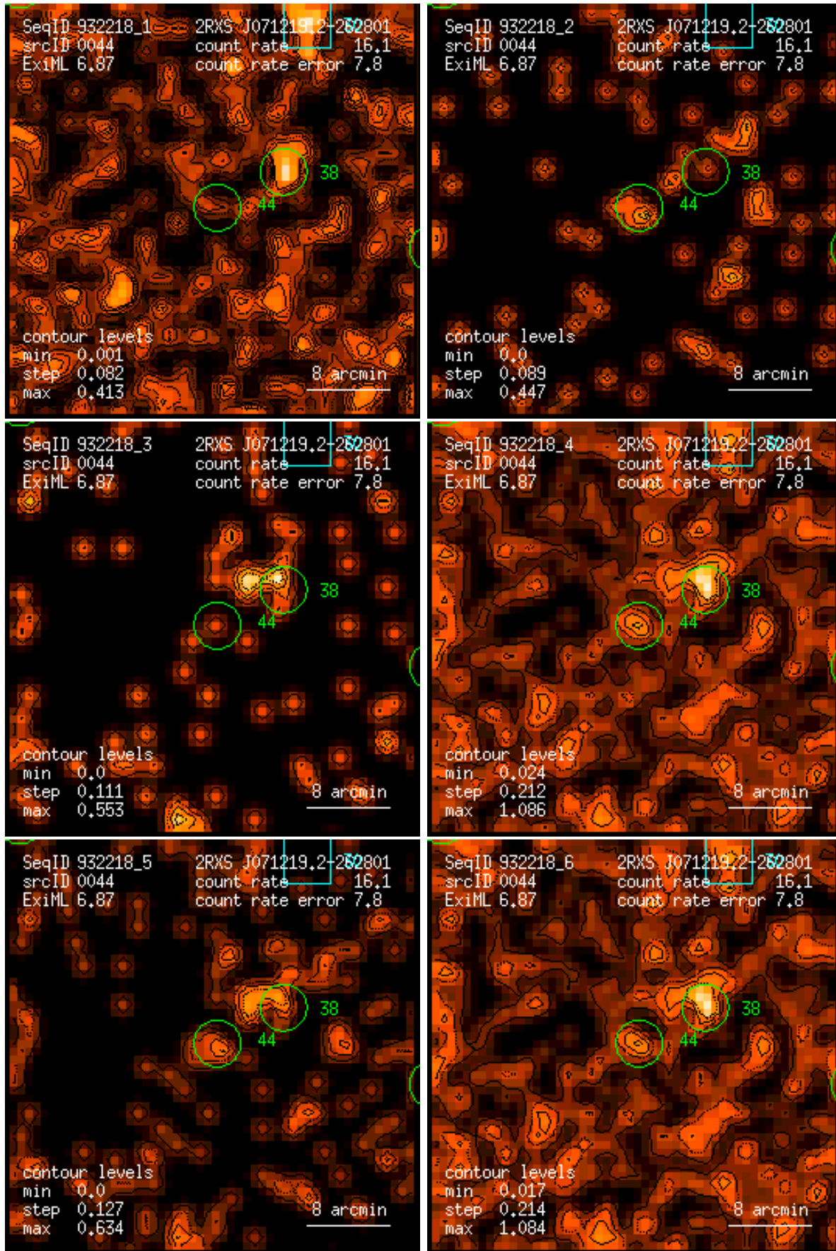
Figure 44: RASS 932218: detection 0044: band rate images, Gaussian filter: (1) PSPC channels 11 – 41, (2) 52 – 90, (3) 91 – 201, (4) 11 – 235, (5) 52 – 201, (6) 11 – 201. Broad band rates in counts/ks. Band rate contour levels in counts/ks/arcmin 2 .
