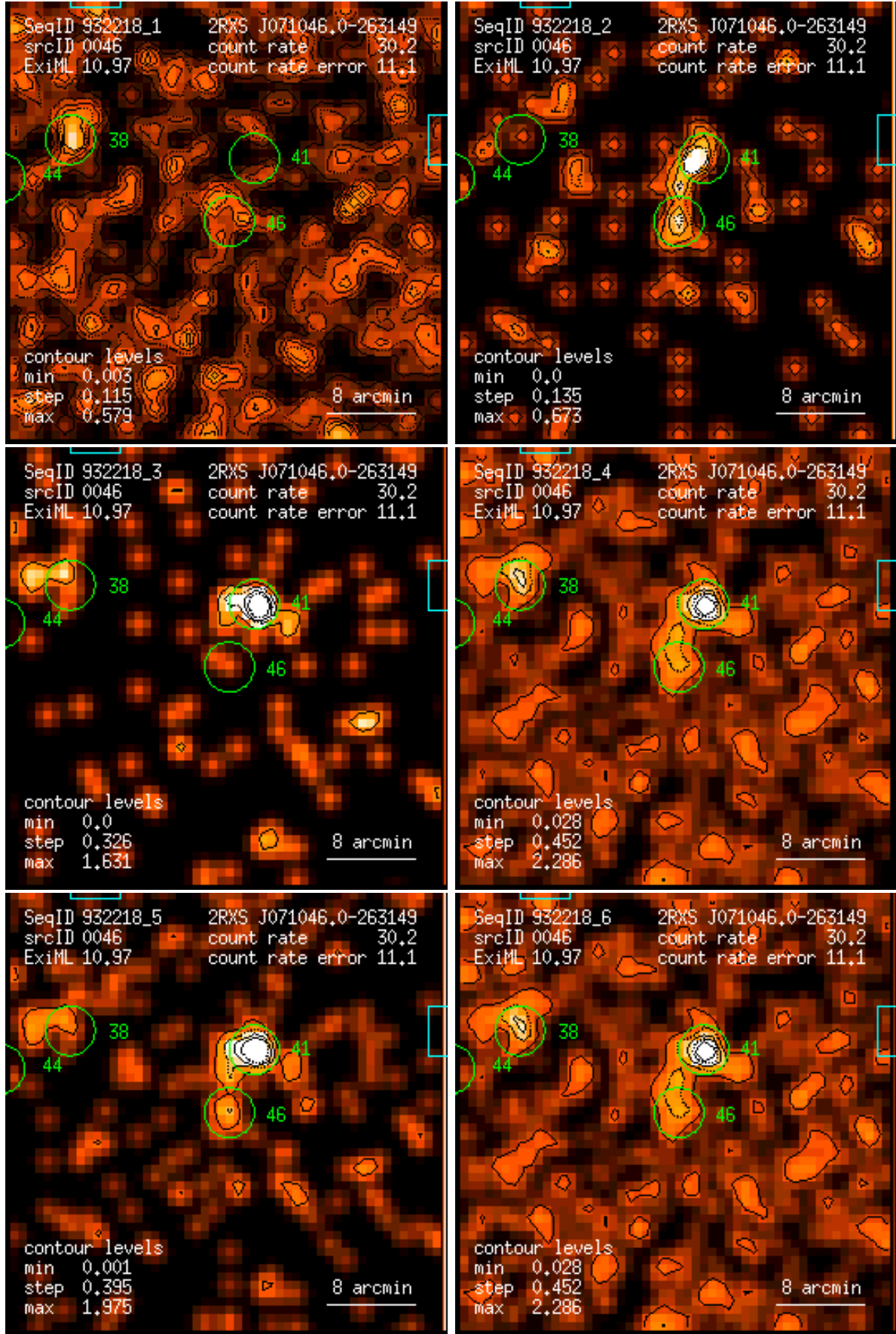
Figure 46: RASS 932218: detection 0046: band rate images, Gaussian filter: (1) PSPC channels 11 – 41, (2) 52 – 90, (3) 91 – 201, (4) 11 – 235, (5) 52 – 201, (6) 11 – 201. Broad band rates in counts/ks. Band rate contour levels in counts/ks/arcmin 2 .
