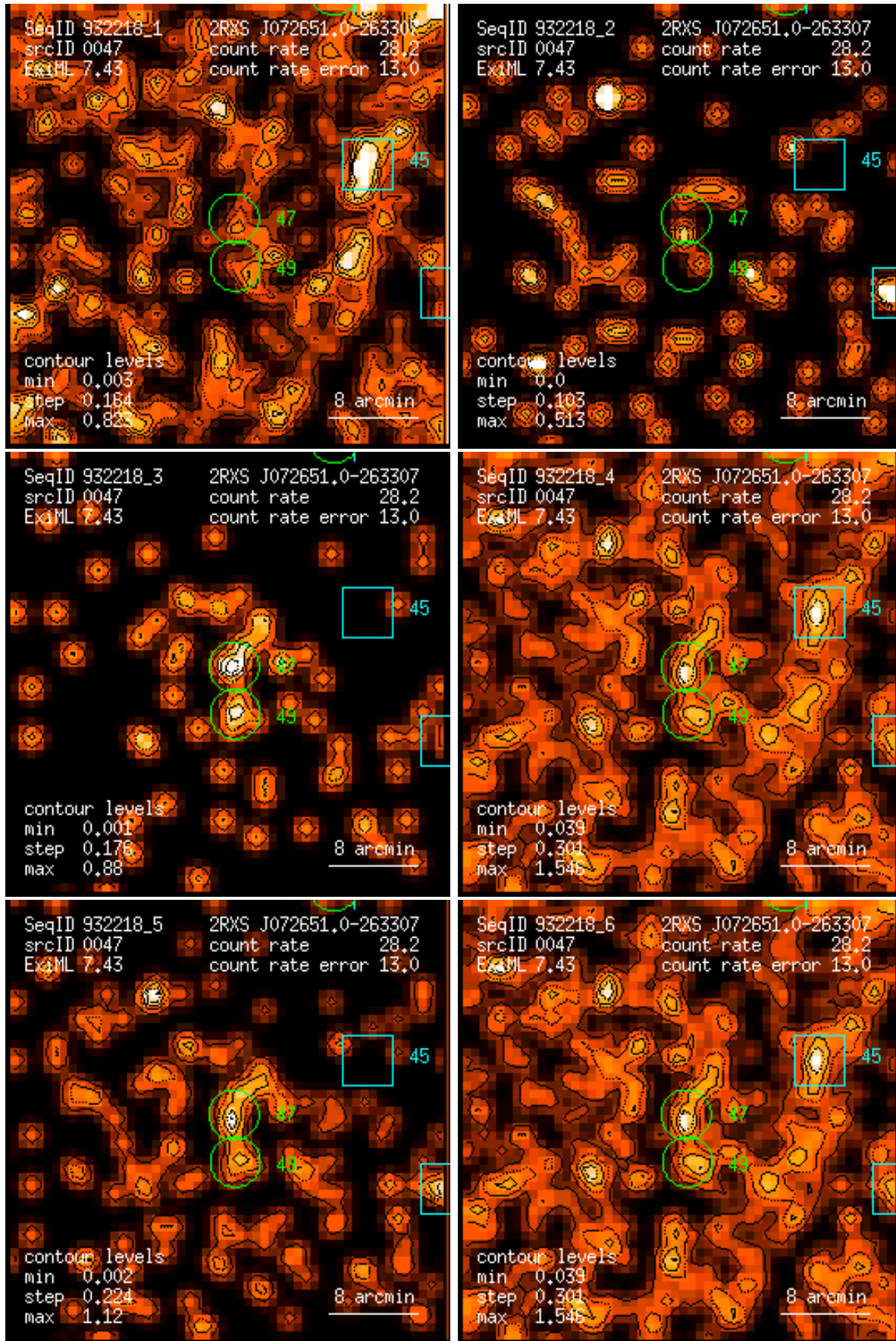
Figure 47: RASS 932218: detection 0047: band rate images, Gaussian filter: (1) PSPC channels 11 – 41, (2) 52 – 90, (3) 91 – 201, (4) 11 – 235, (5) 52 – 201, (6) 11 – 201. Broad band rates in counts/ks. Band rate contour levels in counts/ks/arcmin 2 .
