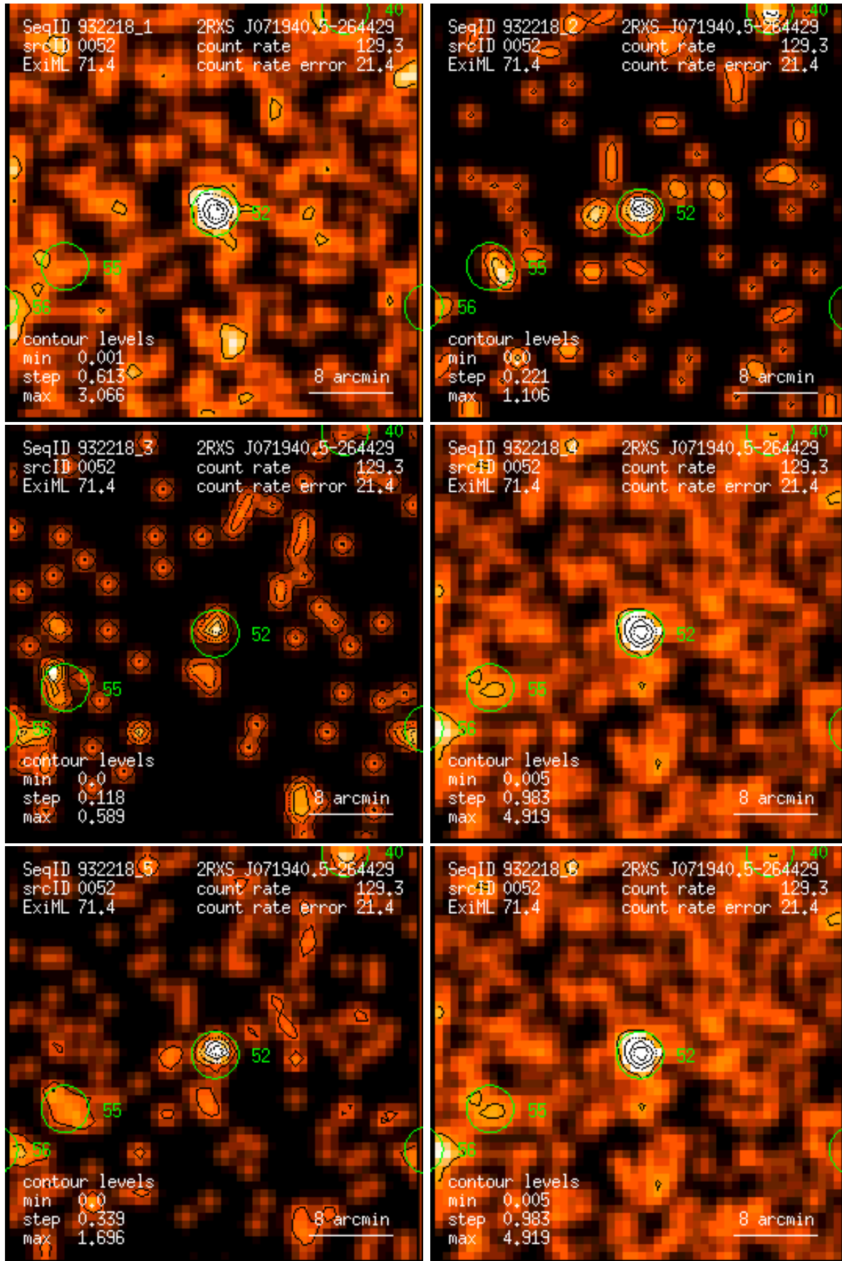
Figure 52: RASS 932218: detection 0052: band rate images, Gaussian filter: (1) PSPC channels 11 – 41, (2) 52 – 90, (3) 91 – 201, (4) 11 – 235, (5) 52 – 201, (6) 11 – 201. Broad band rates in counts/ks. Band rate contour levels in counts/ks/arcmin 2 .
