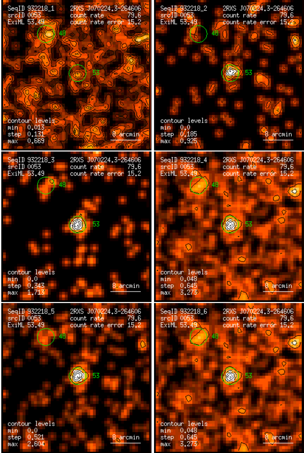
Figure 53: RASS 932218: detection 0053: band rate images, Gaussian filter: (1) PSPC channels 11 – 41, (2) 52 – 90, (3) 91 – 201, (4) 11 – 235, (5) 52 – 201, (6) 11 – 201. Broad band rates in counts/ks. Band rate contour levels in counts/ks/arcmin 2 .
