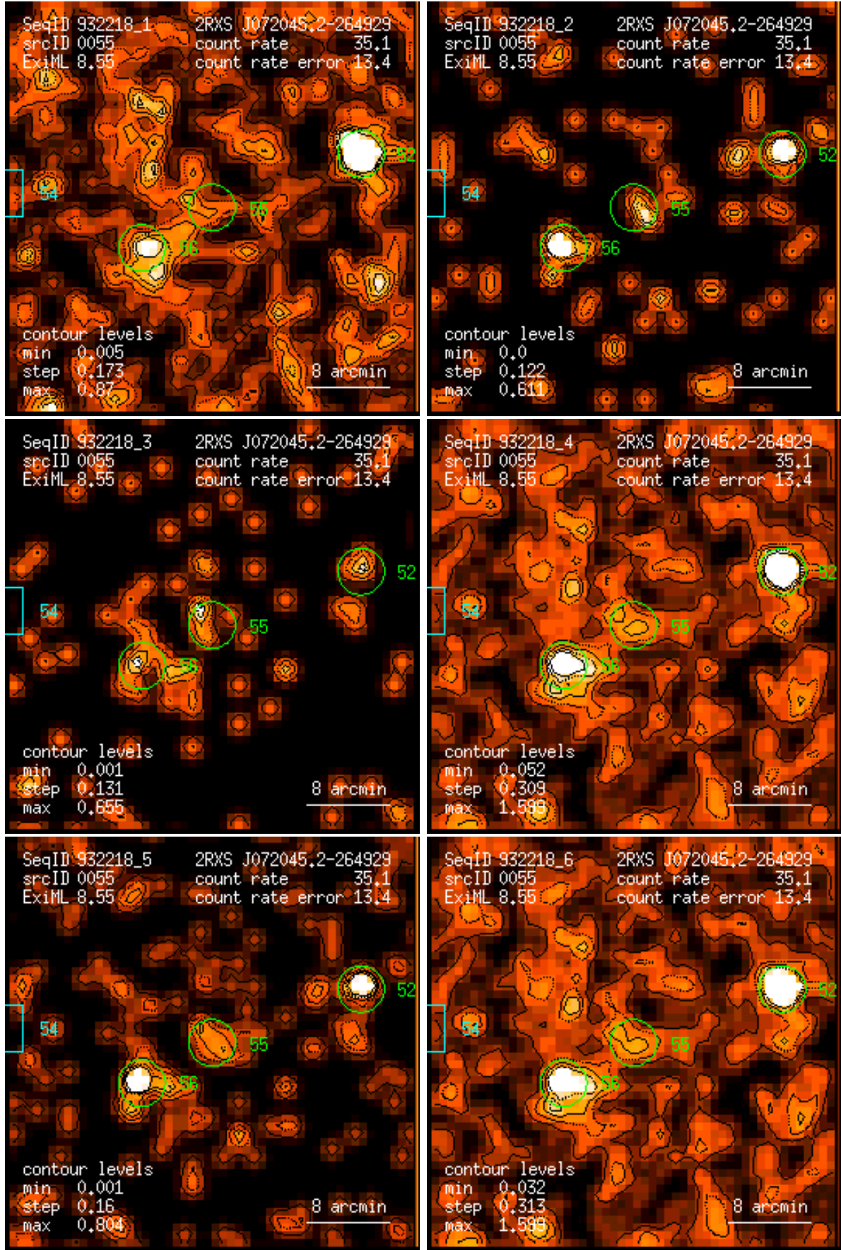
Figure 55: RASS 932218: detection 0055: band rate images, Gaussian filter: (1) PSPC channels 11 – 41, (2) 52 – 90, (3) 91 – 201, (4) 11 – 235, (5) 52 – 201, (6) 11 – 201. Broad band rates in counts/ks. Band rate contour levels in counts/ks/arcmin 2 .
