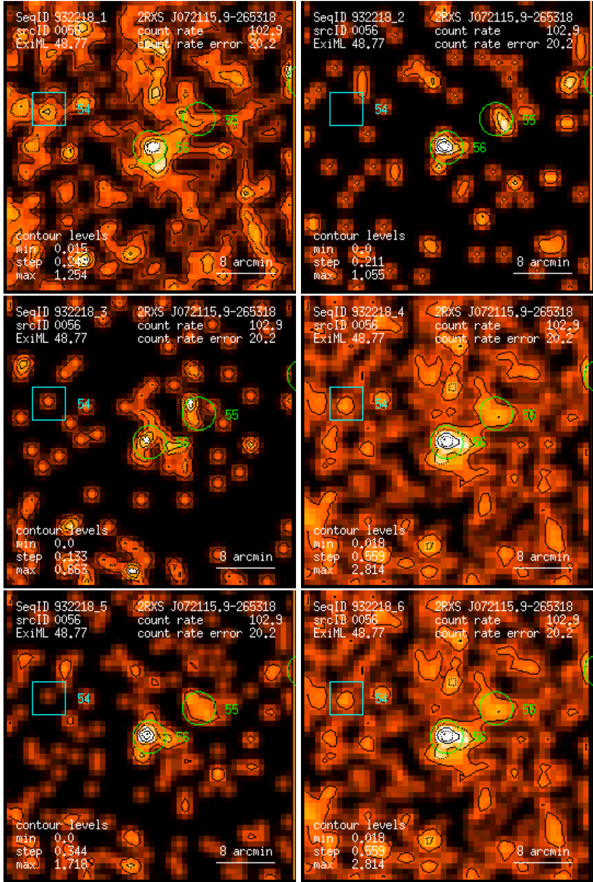
Figure 56: RASS 932218: detection 0056: band rate images, Gaussian filter: (1) PSPC channels 11 – 41, (2) 52 – 90, (3) 91 – 201, (4) 11 – 235, (5) 52 – 201, (6) 11 – 201. Broad band rates in counts/ks. Band rate contour levels in counts/ks/arcmin 2 .
