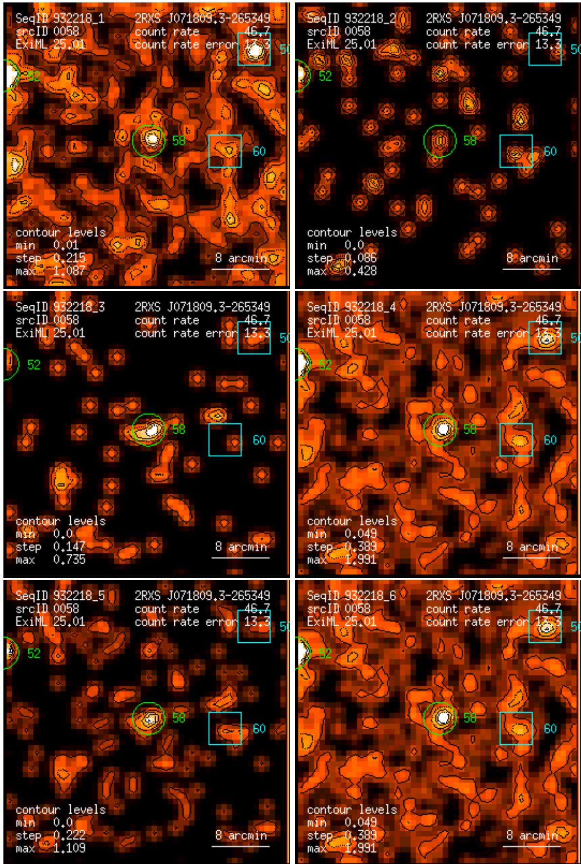
Figure 58: RASS 932218: detection 0058: band rate images, Gaussian filter: (1) PSPC channels 11 – 41, (2) 52 – 90, (3) 91 – 201, (4) 11 – 235, (5) 52 – 201, (6) 11 – 201. Broad band rates in counts/ks. Band rate contour levels in counts/ks/arcmin 2 .
