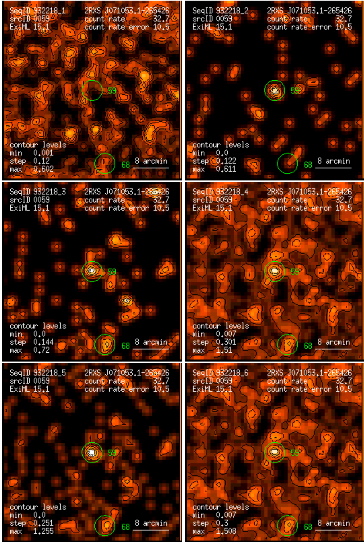
Figure 59: RASS 932218: detection 0059: band rate images, Gaussian filter: (1) PSPC channels 11 – 41, (2) 52 – 90, (3) 91 – 201, (4) 11 – 235, (5) 52 – 201, (6) 11 – 201. Broad band rates in counts/ks. Band rate contour levels in counts/ks/arcmin 2 .
