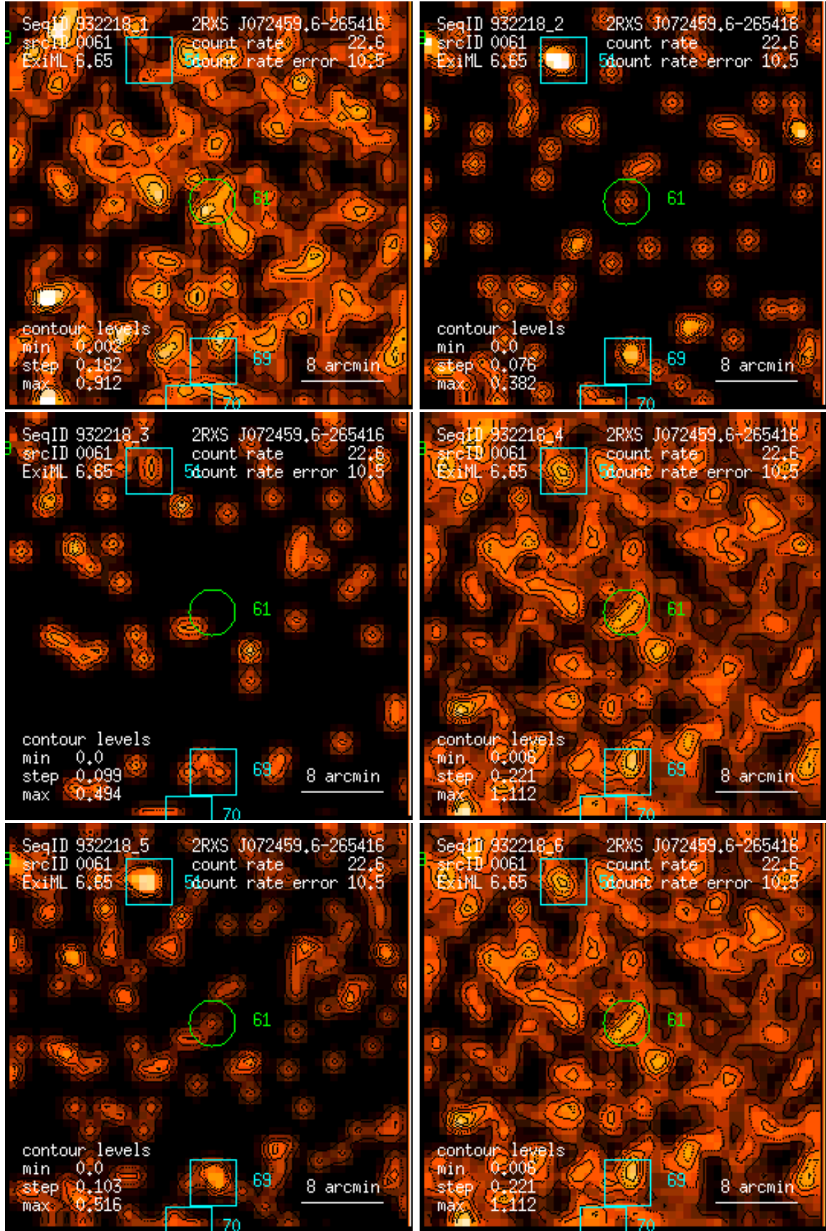
Figure 61: RASS 932218: detection 0061: band rate images, Gaussian filter: (1) PSPC channels 11 – 41, (2) 52 – 90, (3) 91 – 201, (4) 11 – 235, (5) 52 – 201, (6) 11 – 201. Broad band rates in counts/ks. Band rate contour levels in counts/ks/arcmin 2 .
