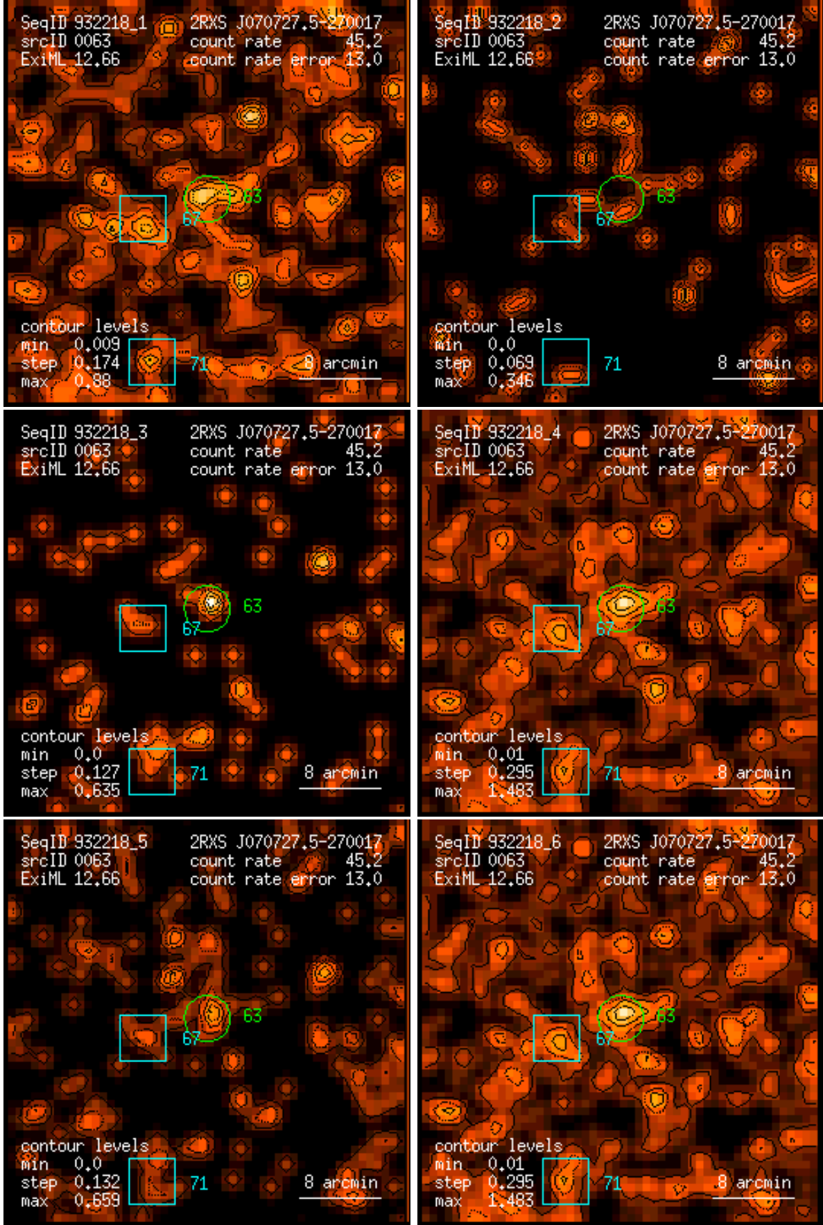
Figure 63: RASS 932218: detection 0063: band rate images, Gaussian filter: (1) PSPC channels 11 – 41, (2) 52 – 90, (3) 91 – 201, (4) 11 – 235, (5) 52 – 201, (6) 11 – 201. Broad band rates in counts/ks. Band rate contour levels in counts/ks/arcmin 2 .
