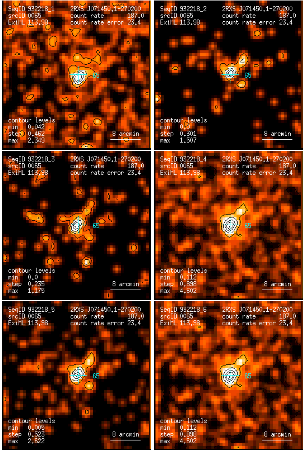
Figure 65: RASS 932218: detection 0065: band rate images, Gaussian filter: (1) PSPC channels 11 – 41, (2) 52 – 90, (3) 91 – 201, (4) 11 – 235, (5) 52 – 201, (6) 11 – 201. Broad band rates in counts/ks. Band rate contour levels in counts/ks/arcmin 2 .
