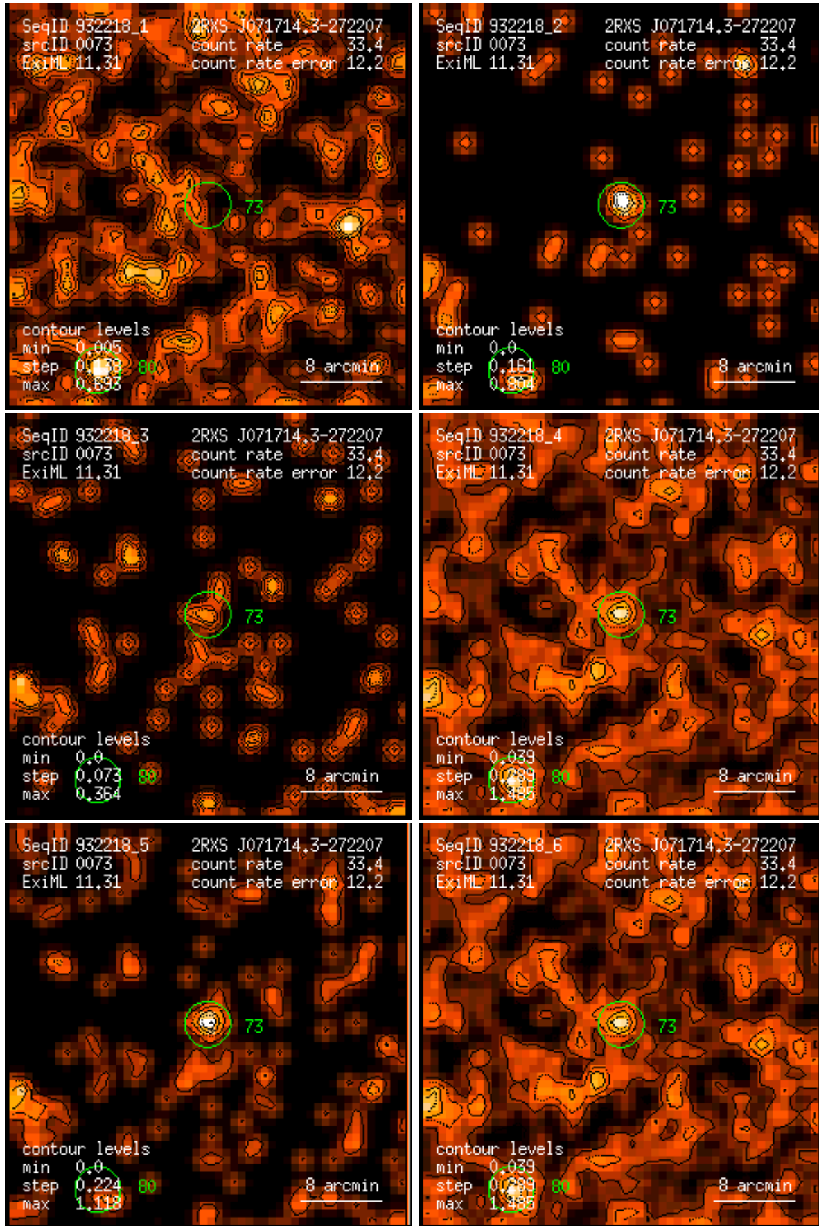
Figure 73: RASS 932218: detection 0073: band rate images, Gaussian filter: (1) PSPC channels 11 – 41, (2) 52 – 90, (3) 91 – 201, (4) 11 – 235, (5) 52 – 201, (6) 11 – 201. Broad band rates in counts/ks. Band rate contour levels in counts/ks/arcmin 2 .
