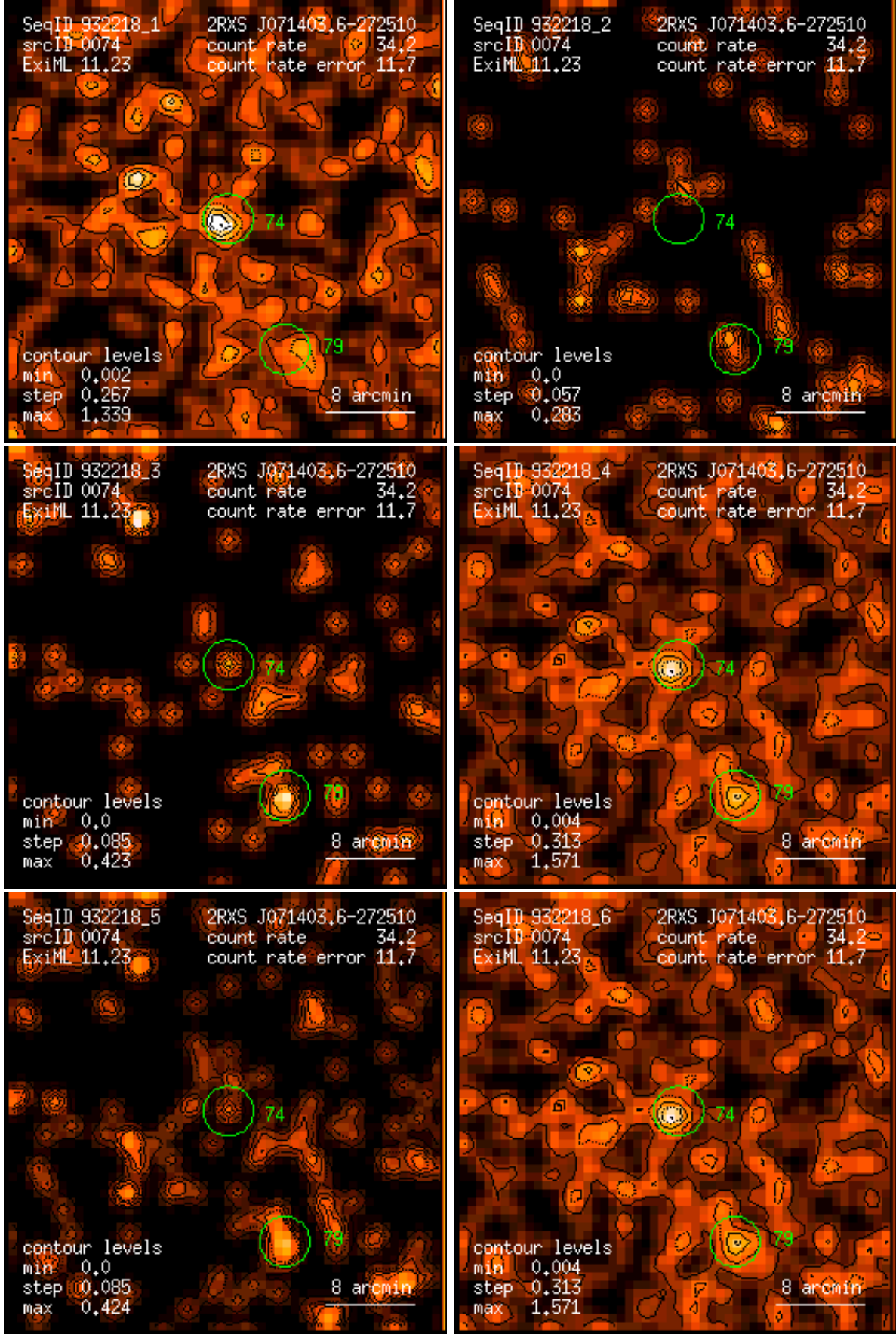
Figure 74: RASS 932218: detection 0074: band rate images, Gaussian filter: (1) PSPC channels 11 – 41, (2) 52 – 90, (3) 91 – 201, (4) 11 – 235, (5) 52 – 201, (6) 11 – 201. Broad band rates in counts/ks. Band rate contour levels in counts/ks/arcmin 2 .
