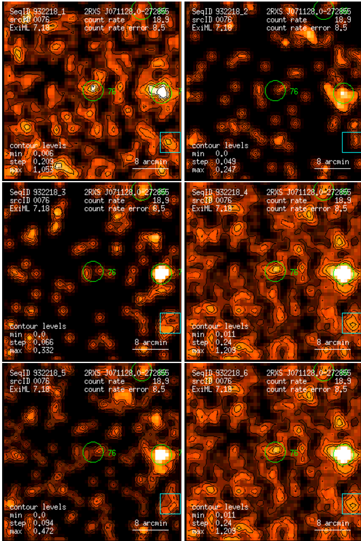
Figure 76: RASS 932218: detection 0076: band rate images, Gaussian filter: (1) PSPC channels 11 – 41, (2) 52 – 90, (3) 91 – 201, (4) 11 – 235, (5) 52 – 201, (6) 11 – 201. Broad band rates in counts/ks. Band rate contour levels in counts/ks/arcmin 2 .
