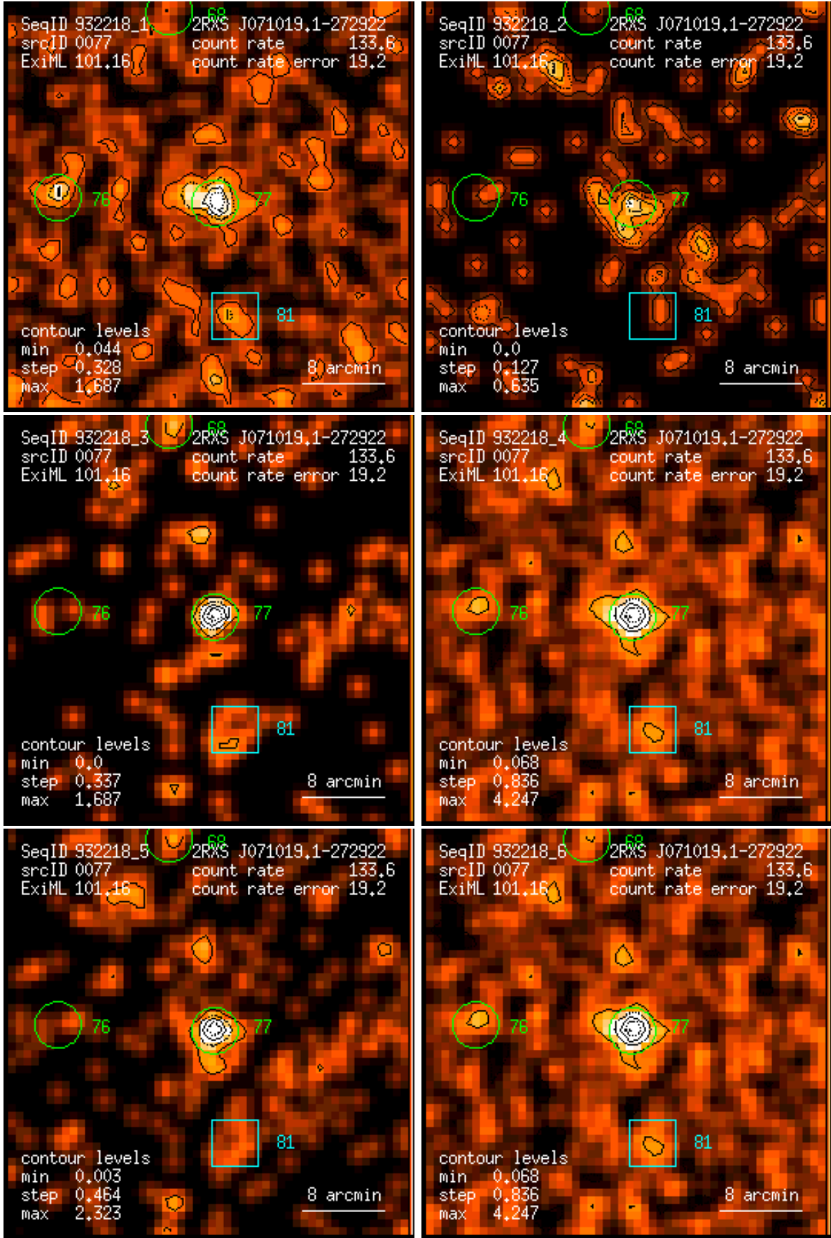
Figure 77: RASS 932218: detection 0077: band rate images, Gaussian filter: (1) PSPC channels 11 – 41, (2) 52 – 90, (3) 91 – 201, (4) 11 – 235, (5) 52 – 201, (6) 11 – 201. Broad band rates in counts/ks. Band rate contour levels in counts/ks/arcmin 2 .
