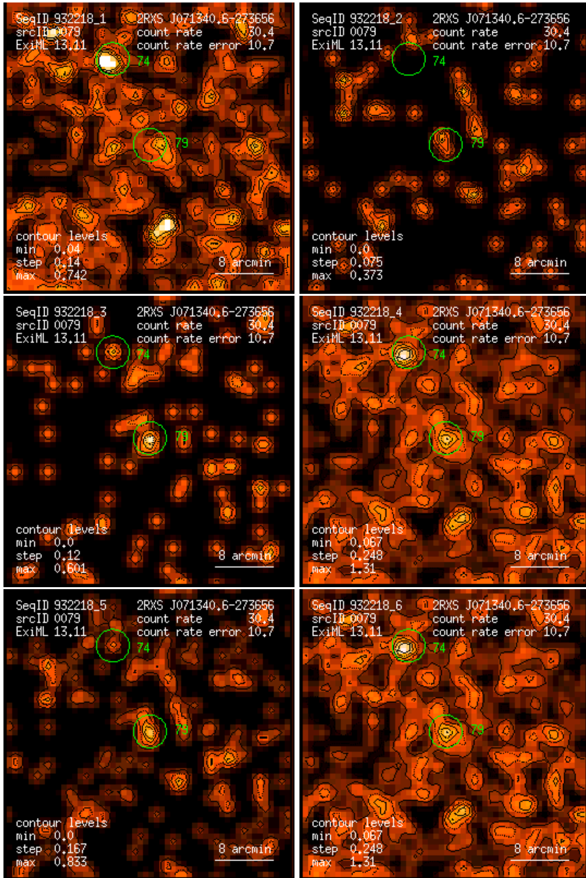
Figure 79: RASS 932218: detection 0079: band rate images, Gaussian filter: (1) PSPC channels 11 – 41, (2) 52 – 90, (3) 91 – 201, (4) 11 – 235, (5) 52 – 201, (6) 11 – 201. Broad band rates in counts/ks. Band rate contour levels in counts/ks/arcmin 2 .
