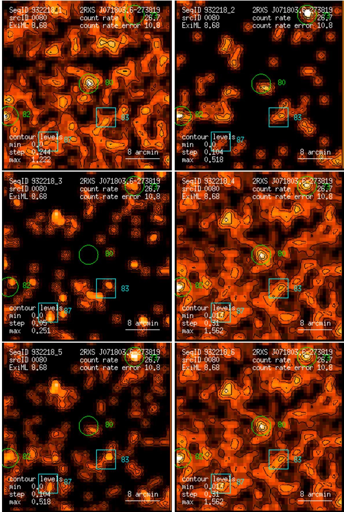
Figure 80: RASS 932218: detection 0080: band rate images, Gaussian filter: (1) PSPC channels 11 – 41, (2) 52 – 90, (3) 91 – 201, (4) 11 – 235, (5) 52 – 201, (6) 11 – 201. Broad band rates in counts/ks. Band rate contour levels in counts/ks/arcmin 2 .
