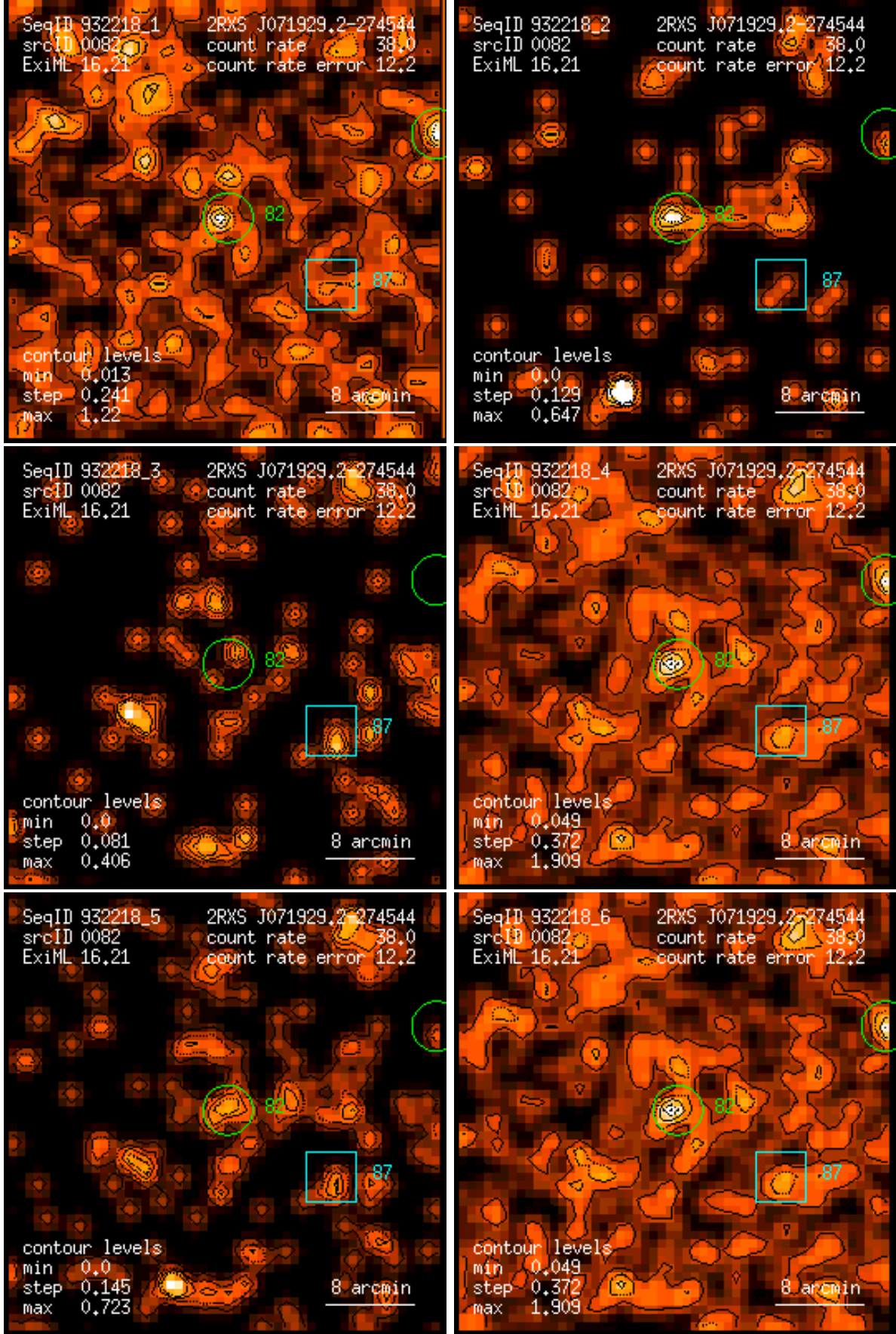
Figure 82: RASS 932218: detection 0082: band rate images, Gaussian filter: (1) PSPC channels 11 – 41, (2) 52 – 90, (3) 91 – 201, (4) 11 – 235, (5) 52 – 201, (6) 11 – 201. Broad band rates in counts/ks. Band rate contour levels in counts/ks/arcmin 2 .
