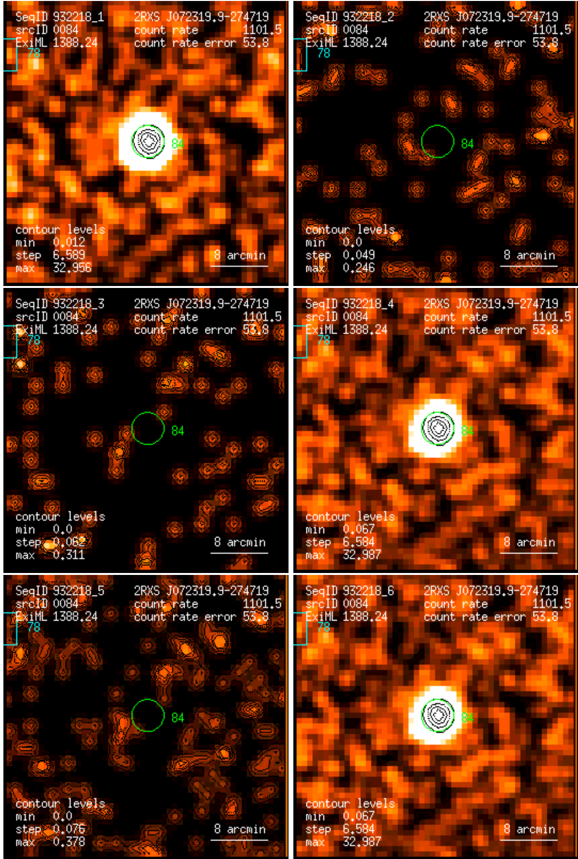
Figure 84: RASS 932218: detection 0084: band rate images, Gaussian filter: (1) PSPC channels 11 – 41, (2) 52 – 90, (3) 91 – 201, (4) 11 – 235, (5) 52 – 201, (6) 11 – 201. Broad band rates in counts/ks. Band rate contour levels in counts/ks/arcmin 2 .
