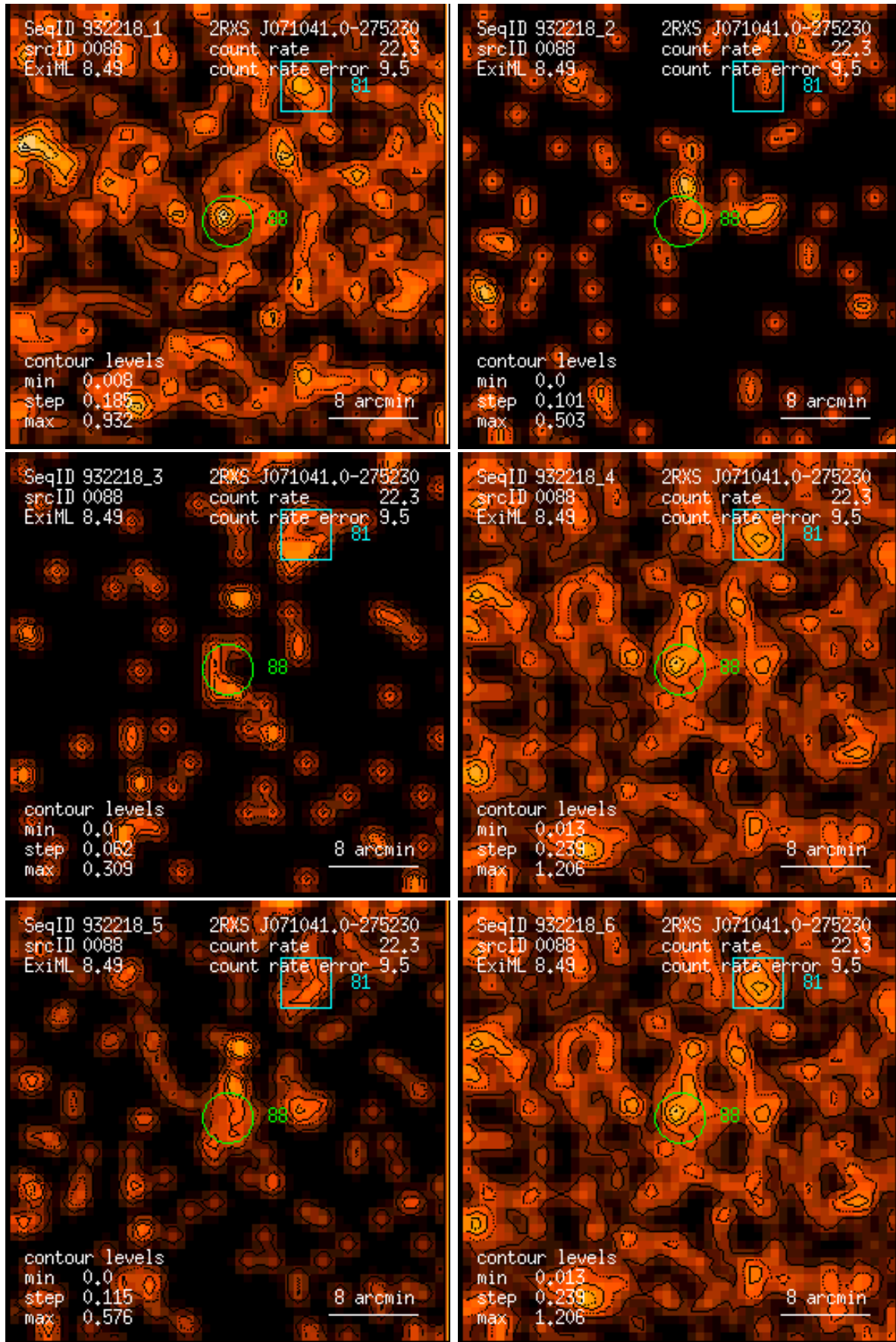
Figure 88: RASS 932218: detection 0088: band rate images, Gaussian filter: (1) PSPC channels 11 – 41, (2) 52 – 90, (3) 91 – 201, (4) 11 – 235, (5) 52 – 201, (6) 11 – 201. Broad band rates in counts/ks. Band rate contour levels in counts/ks/arcmin 2 .
