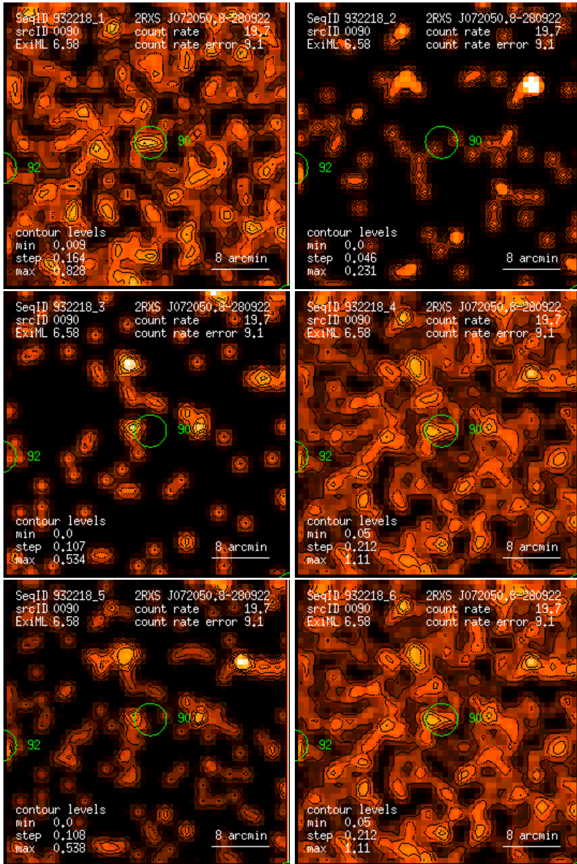
Figure 90: RASS 932218: detection 0090: band rate images, Gaussian filter: (1) PSPC channels 11 – 41, (2) 52 – 90, (3) 91 – 201, (4) 11 – 235, (5) 52 – 201, (6) 11 – 201. Broad band rates in counts/ks. Band rate contour levels in counts/ks/arcmin 2 .
