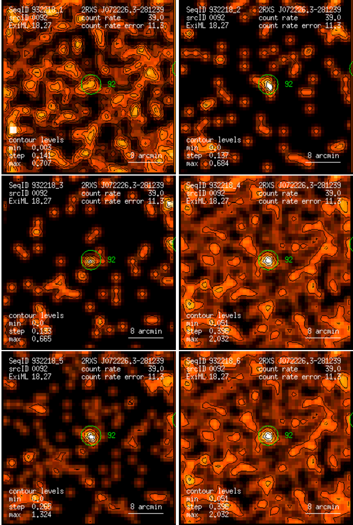
Figure 92: RASS 932218: detection 0092: band rate images, Gaussian filter: (1) PSPC channels 11 – 41, (2) 52 – 90, (3) 91 – 201, (4) 11 – 235, (5) 52 – 201, (6) 11 – 201. Broad band rates in counts/ks. Band rate contour levels in counts/ks/arcmin 2 .
