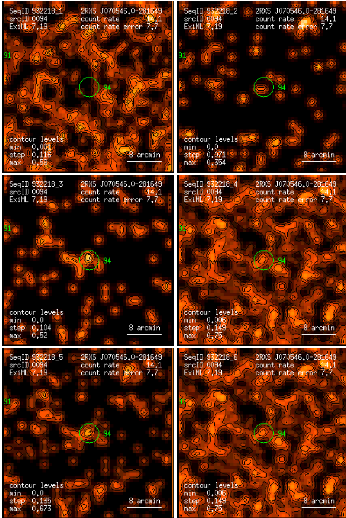
Figure 94: RASS 932218: detection 0094: band rate images, Gaussian filter: (1) PSPC channels 11 – 41, (2) 52 – 90, (3) 91 – 201, (4) 11 – 235, (5) 52 – 201, (6) 11 – 201. Broad band rates in counts/ks. Band rate contour levels in counts/ks/arcmin 2 .
