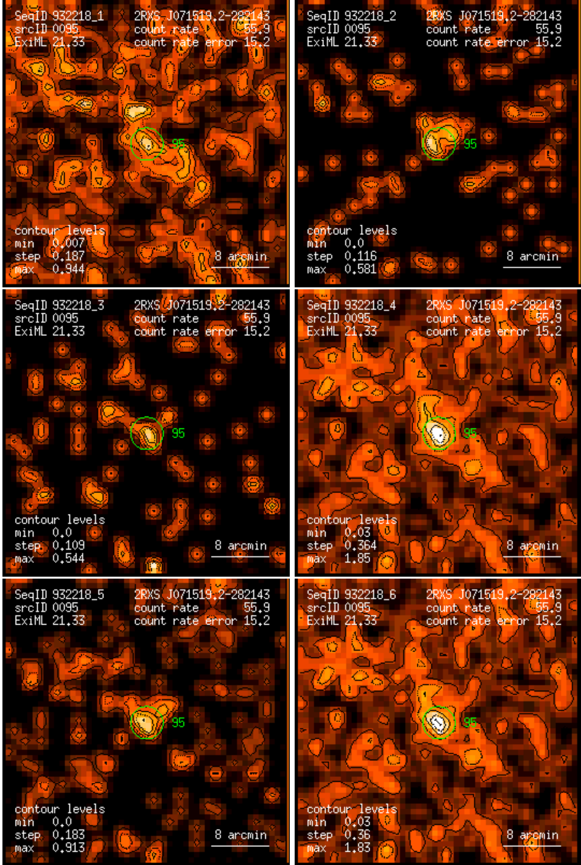
Figure 95: RASS 932218: detection 0095: band rate images, Gaussian filter: (1) PSPC channels 11 – 41, (2) 52 – 90, (3) 91 – 201, (4) 11 – 235, (5) 52 – 201, (6) 11 – 201. Broad band rates in counts/ks. Band rate contour levels in counts/ks/arcmin 2 .
