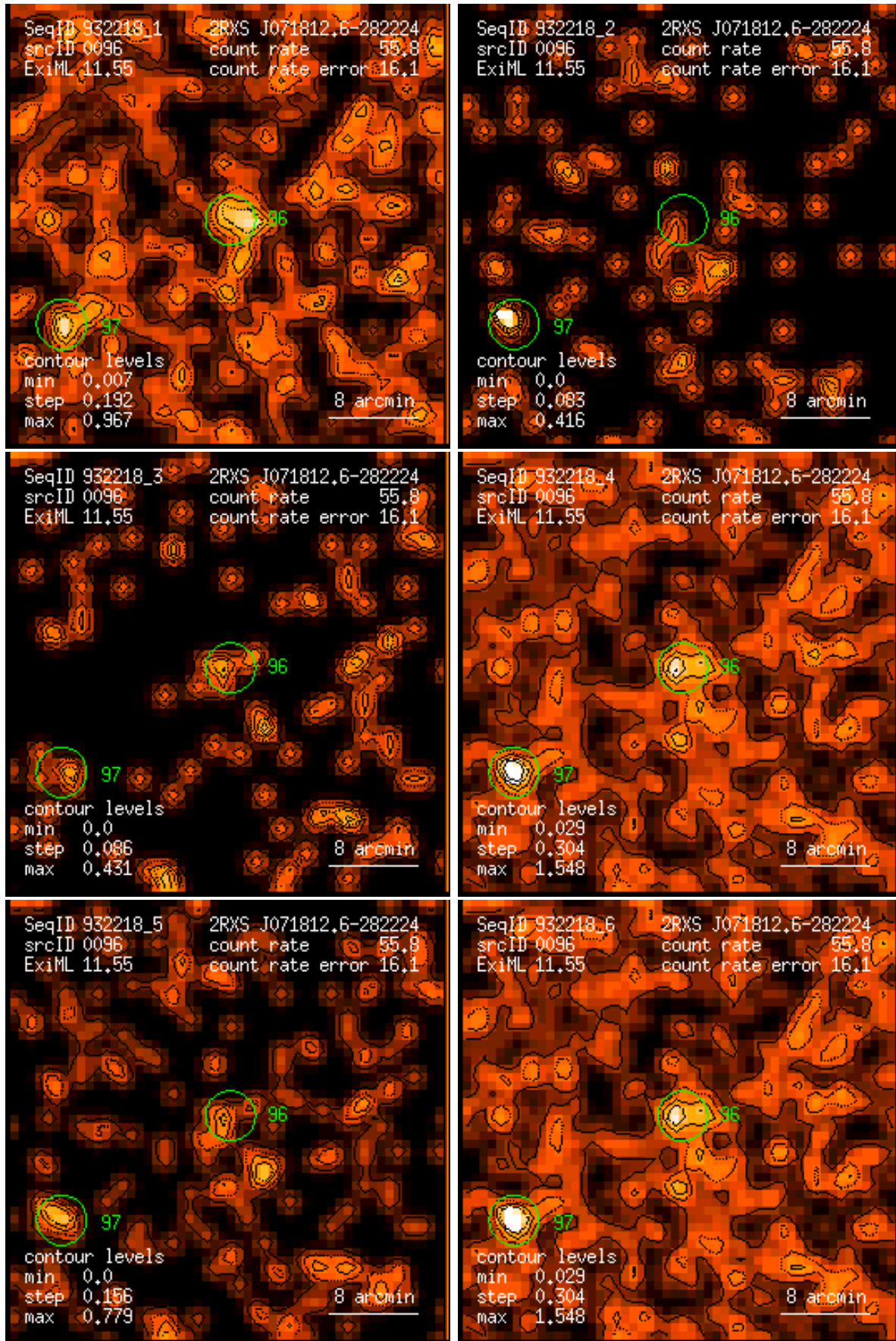
Figure 96: RASS 932218: detection 0096: band rate images, Gaussian filter: (1) PSPC channels 11 – 41, (2) 52 – 90, (3) 91 – 201, (4) 11 – 235, (5) 52 – 201, (6) 11 – 201. Broad band rates in counts/ks. Band rate contour levels in counts/ks/arcmin 2 .
