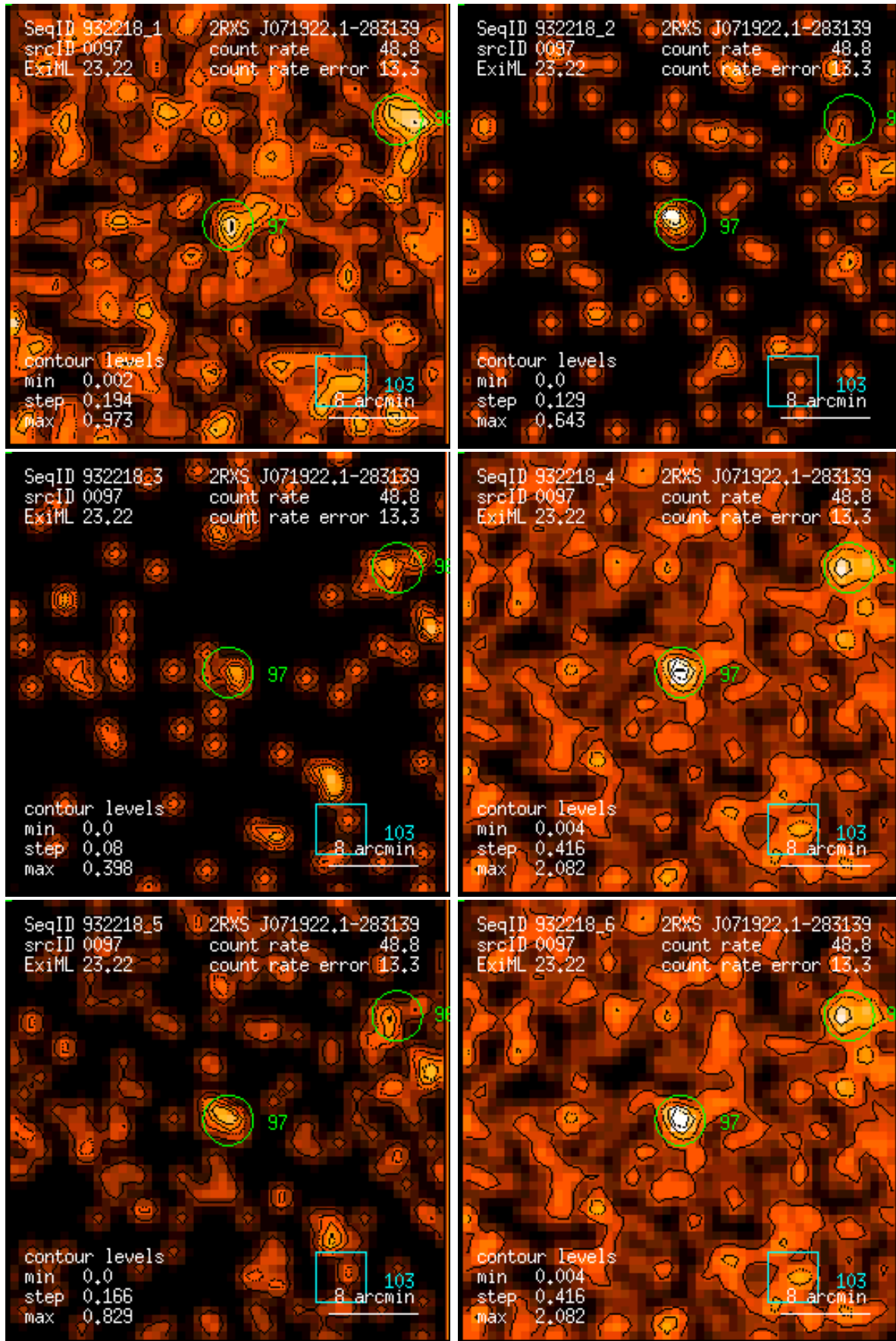
Figure 97: RASS 932218: detection 0097: band rate images, Gaussian filter: (1) PSPC channels 11 – 41, (2) 52 – 90, (3) 91 – 201, (4) 11 – 235, (5) 52 – 201, (6) 11 – 201. Broad band rates in counts/ks. Band rate contour levels in counts/ks/arcmin 2 .
