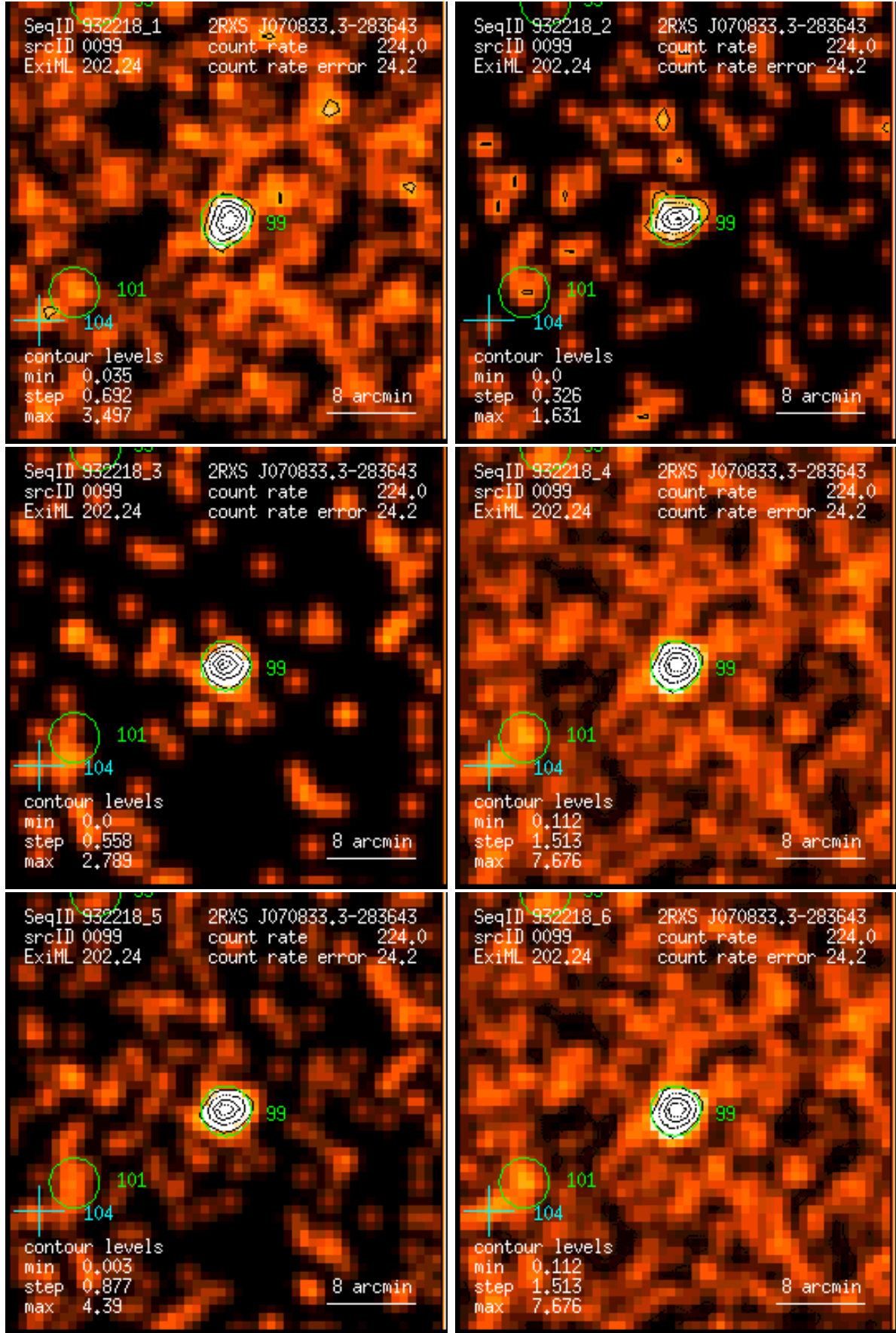
Figure 99: RASS 932218: detection 0099: band rate images, Gaussian filter: (1) PSPC channels 11 – 41, (2) 52 – 90, (3) 91 – 201, (4) 11 – 235, (5) 52 – 201, (6) 11 – 201. Broad band rates in counts/ks. Band rate contour levels in counts/ks/arcmin 2 .
