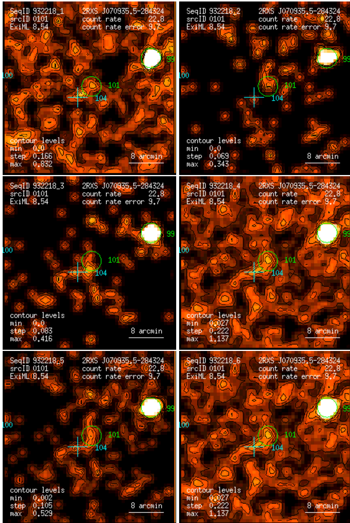
Figure 101: RASS 932218: detection 0101: band rate images, Gaussian filter: (1) PSPC channels 11 – 41, (2) 52 – 90, (3) 91 – 201, (4) 11 – 235, (5) 52 – 201, (6) 11 – 201. Broad band rates in counts/ks. Band rate contour levels in counts/ks/arcmin 2 .
