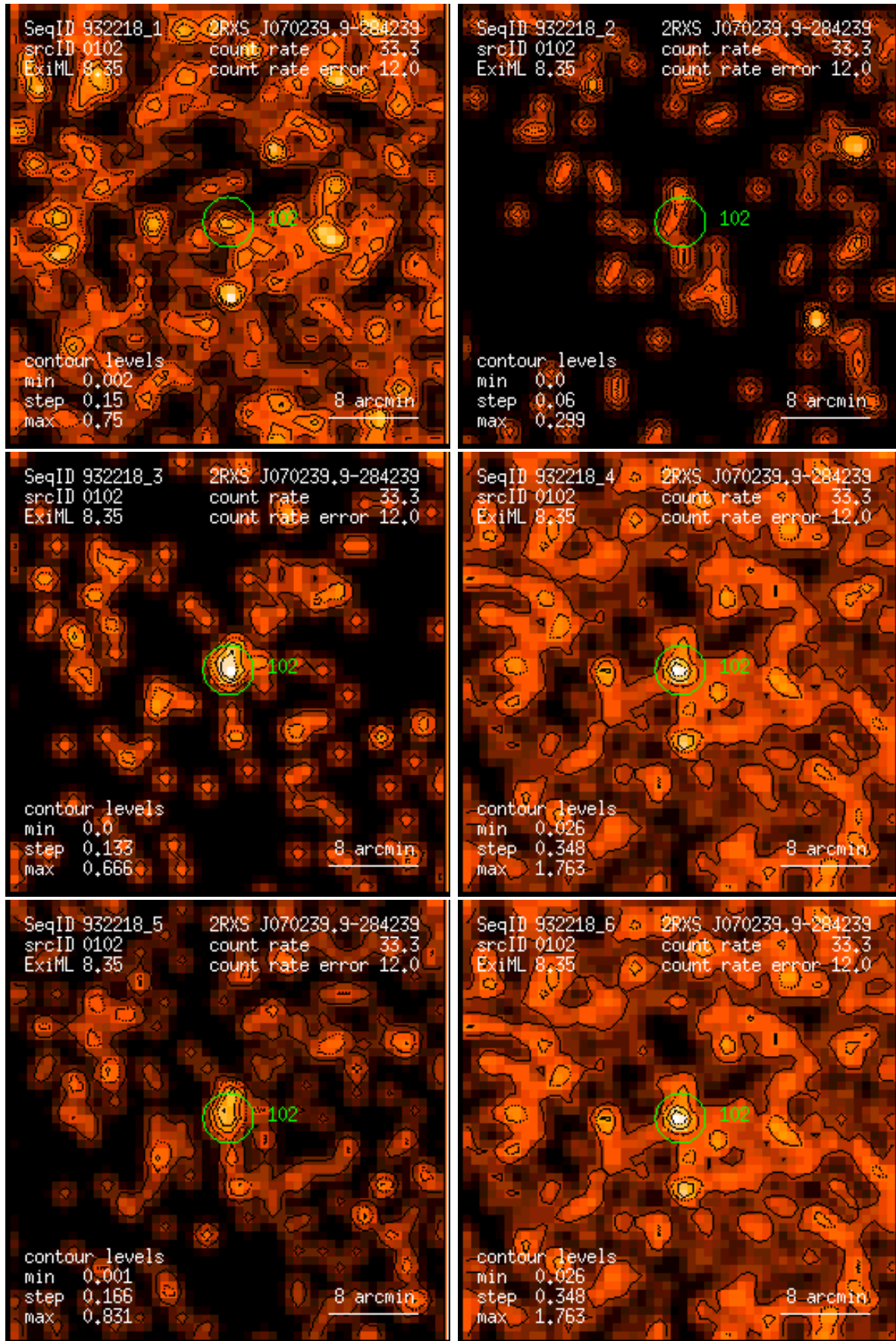
Figure 102: RASS 932218: detection 0102: band rate images, Gaussian filter: (1) PSPC channels 11 – 41, (2) 52 – 90, (3) 91 – 201, (4) 11 – 235, (5) 52 – 201, (6) 11 – 201. Broad band rates in counts/ks. Band rate contour levels in counts/ks/arcmin 2 .
