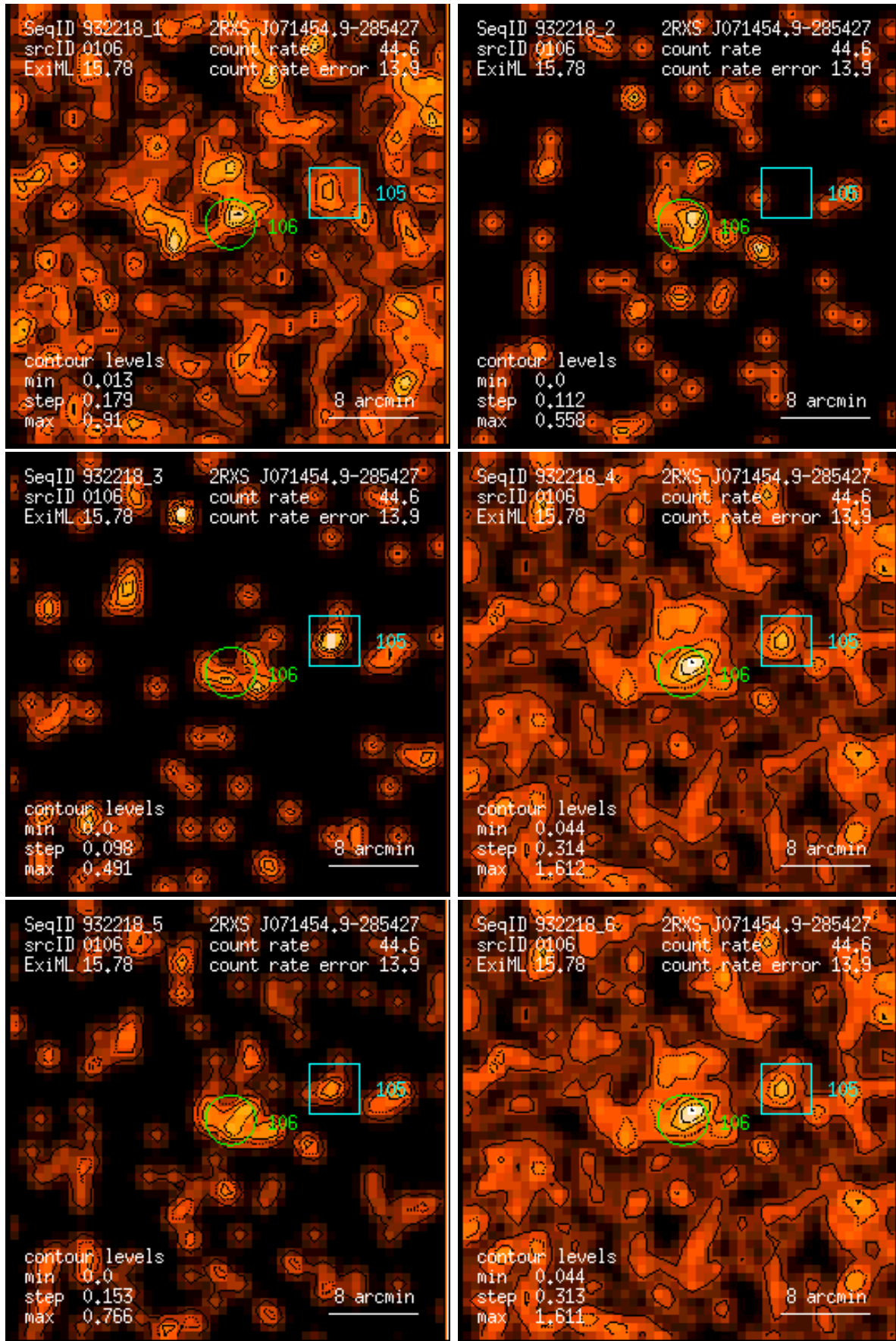
Figure 106: RASS 932218: detection 0106: band rate images, Gaussian filter: (1) PSPC channels 11 – 41, (2) 52 – 90, (3) 91 – 201, (4) 11 – 235, (5) 52 – 201, (6) 11 – 201. Broad band rates in counts/ks. Band rate contour levels in counts/ks/arcmin 2 .
